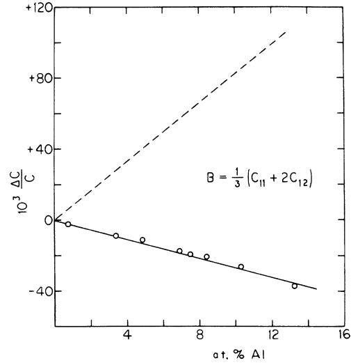
FIG. 4. Fractional change in the bulk modulus B = \frac{1}{3}(C_{11} + 2C_{12}) of \alpha -Cu-Al extrapolated to 0^\circ\text{K} . Dashed line represents the change that would be observed upon alloying at constant volume.
