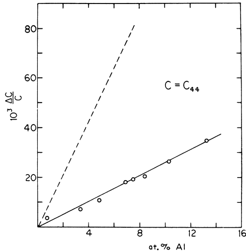
FIG. 2. Fractional change in the elastic shear coefficient C = C_{44} of \alpha -Cu-Al extrapolated to 0^\circ\text{K} . Dashed line represents the change that would be observed upon alloying at constant volume.
