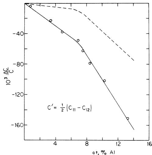
FIG. 3. Fractional change in the elastic shear coefficient C' = \frac{1}{2}(C_{11} - C_{12}) of \alpha -Cu-Al extrapolated to 0^\circ\text{K} . Data have been fit with two straight lines to illustrate the greater rate of decrease of C' above 7 at.% Al. Dashed line represents the change that would be observed upon alloying at constant volume.
