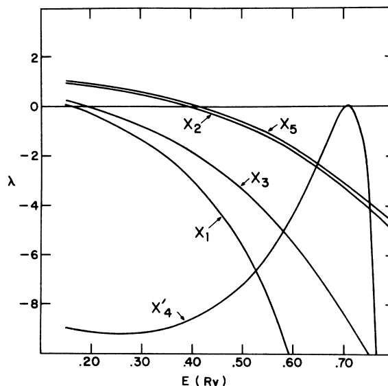
FIG. 1. \lambda -vs- E plot at the X point for Cu.
