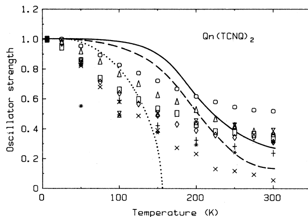
FIG. 7. Temperature dependence of the oscillator strength of eight a_g modes in \text{Qn}(\text{TCNQ})_2 : \nu_3 = 1605 \text{ cm}^{-1} ( \square ), \nu_4 = 1425 \text{ cm}^{-1} ( \circ ), \nu_5 = 1195 \text{ cm}^{-1} ( \triangle ), \nu_6 = 950 \text{ cm}^{-1} ( \times ), \nu_7 = 691 \text{ cm}^{-1} ( \diamond ), \nu_8 = 600 \text{ cm}^{-1} ( * ), \nu_9 = 306 \text{ cm}^{-1} ( + ), and \nu_{10} = 124 \text{ cm}^{-1} ( \otimes ). The curves shown represent the calculated gap for \text{Qn}(\text{TCNQ})_2 from Ref. 21: the dotted line for \Delta_e = 0 \text{ K} (i.e., no external potential), the dashed line for \Delta_e = 10 \text{ K} , and the solid line for \Delta_e = 25 \text{ K} .
