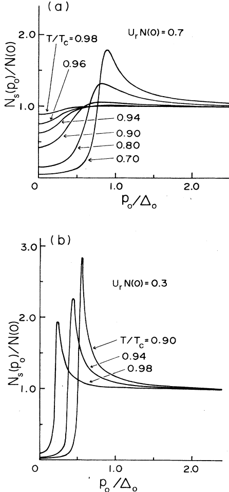
FIG. 2. Energy dependence of the density of states for various temperatures. (a) U_r N(0) = 0.7 , (b) U_r N(0) = 0.3 .
