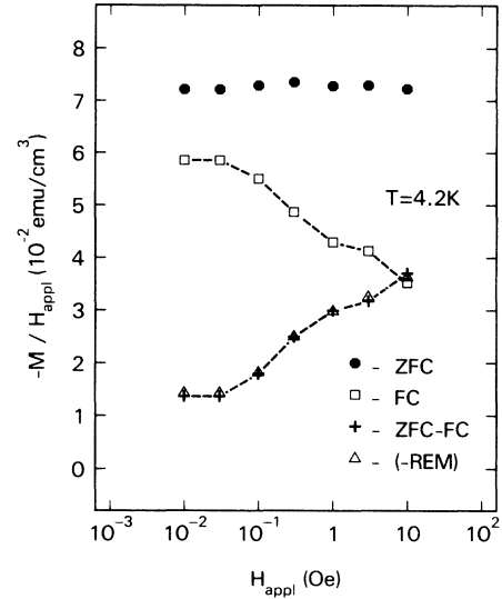
FIG. 3. Low-temperature zero-field-cooled (ZFC), field-cooled (FC), and remanent (REM) moments, normalized by applied field H_{\text{appl}} , for a high-density Y-Ba-Cu-O ceramic (Ref. 18) (see Table I). The difference of M_{\text{FC}} and M_{\text{ZFC}} is compared to M_{\text{rem}} ; they are closely equal.
