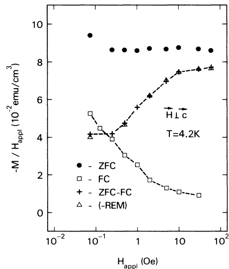
FIG. 4. Low-temperature zero-field-cooled (ZFC), field-cooled (FC), and remanent (REM) moments, normalized by applied field H_{\text{appl}} , for a 0.25-mg Y-Ba-Cu-O crystal (Ref. 19) (see Table I) with field applied perpendicular to the c axis. The difference of M_{\text{FC}} and M_{\text{ZFC}} is compared to M_{\text{rem}} ; they are closely equal.
