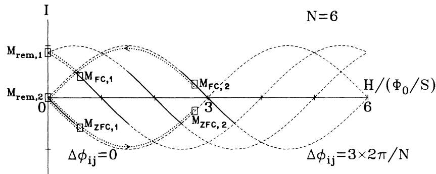
FIG. 8. Current for the first four flux states of a six-member Ebner-Stroud (Ref. 10) loop. Two cases for determining the FC, ZFC, and REM moments are illustrated for H/(\Phi_0/S) equal to 0.6 and 2.75. The first case, labeled 1, corresponds to H close to zero, so that M_{rem} closely approximates M_{FC} - M_{ZFC} . The second case, labeled 2, corresponds to the limit for true glassy behavior in which M_{rem} has no simple relation to M_{FC} - M_{ZFC} .
