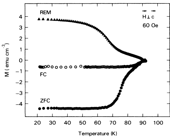
FIG. 2. Zero-field-cooled (ZFC), field-cooled (FC), and remanent (REM) moments as a function of temperature, for a 0.25-mg Y-Ba-Cu-O crystal (Ref. 19) (see Table I) with 60-Oe field applied perpendicular to the c axis. There is a noteworthy broadening of the transition as compared to the 1-Oe data in Fig. 6.
