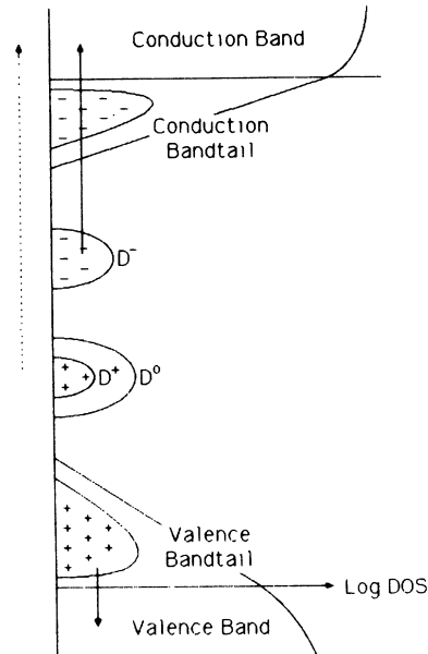
FIG. 6. Diagram of states in the gap in which PM active transitions are shown. The solid lines correspond to the transitions associated with an absorptive photomodulated signal while the dashed line corresponds to the transition which is reduced by excitation resulting in the bleached 1.06-eV signal.
