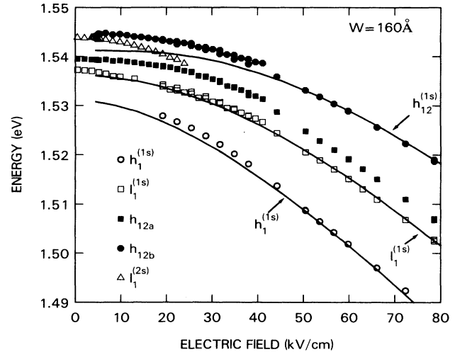
FIG. 2. Energies of some of the exciton peaks in Fig. 1 as a function of electric field. Solid lines are numerically calculated energies of h_1^{(1s)} , l_1^{(1s)} , and h_{12}^{(1s)} in the envelope-function approximation.
