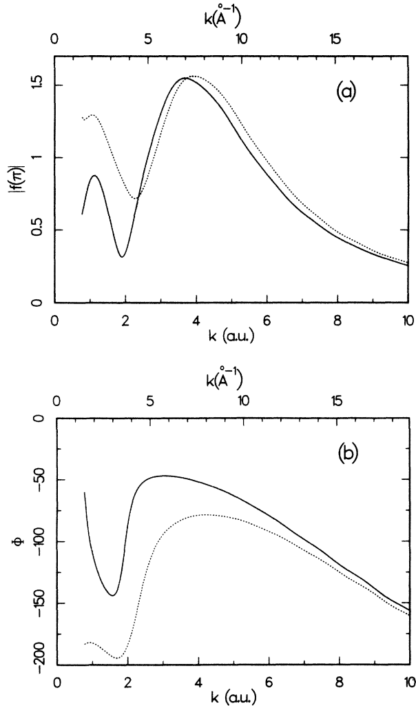
FIG. 1. (a) Modulus and (b) phase of the effective backscattering amplitude \tilde{f}(\pi, R) vs wave number k beyond k_F for the first (solid line) and fourth (dotted line) neighbors in Cu ( R_1=4.80 and R_4=2R_1=9.60 bohrs) and for the standard backscattering amplitude, f(\pi)=\tilde{f}(\pi, \infty) (dashed curves). For other R , \tilde{f}(\pi, R) is given approximately by interpolation in 1/R .
