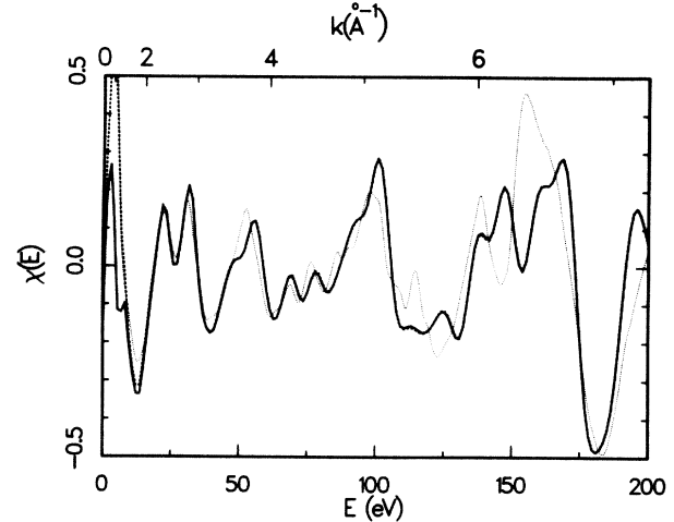
FIG. 2. K -shell EXAFS spectrum \chi(E) for Cu as calculated using SWA formulae for single-scattering and shadowing corrections (solid line), the corresponding exact formulae (Ref. 7) (dashed line), and the LAPW band-structure approach (Ref. 10) (dotted line). All spectra are broadened by a Lorentzian of half-width \eta=4 eV. The absorption edge begins at \approx 7 eV.
