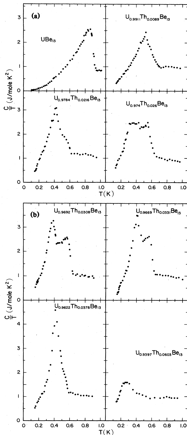
FIG. 2. (a),(b) Specific heat of various U_{1-x}Th_xBe_{13} compounds, plotted as c_p/T vs T for temperatures between 0.15 and 1 K.
