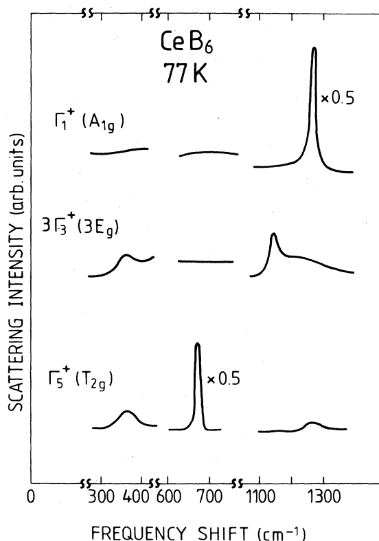
FIG. 3. Symmetry analysis of the \Gamma_8 - \Gamma_7 CEF transition and the Raman-active phonons of \text{CeB}_6 .
