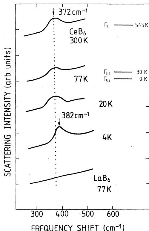
FIG. 2. Raman scattering intensities of \text{CeB}_6 and \text{LaB}_6 at different temperatures showing the \text{Ce}^{3+} \Gamma_8 - \Gamma_7 CEF transition. Inset: Derived CEF level scheme of \text{CeB}_6 .
