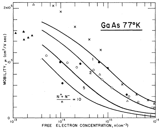
FIG. 3. Electron drift mobility vs free-electron concentration at 77 °K. The curves are calculated for compensation ratios of 1, 2, 5, and 10. Experimental Hall mobilities appear as data points: \Delta , Ref. 18; \blacktriangle , Ref. 22; \bullet , Ref. 23; \times , Ref. 32; \circ , Ref. 33.
