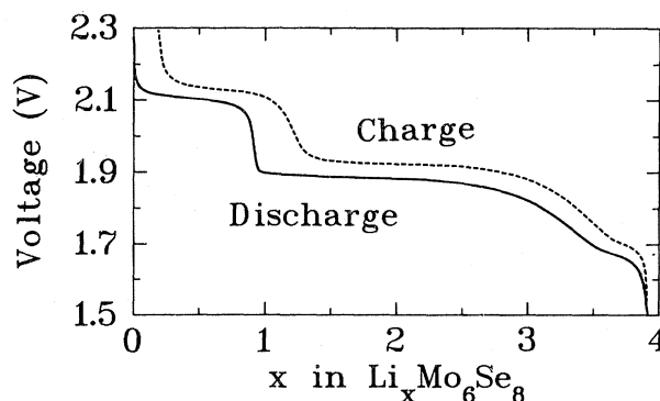
FIG. 1. V(x) for a \text{Li}/\text{Li}_x\text{Mo}_6\text{Se}_8 cell.
