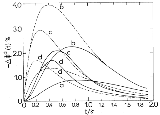
FIG. 1. Delayed fluorescence decay signal -\Delta\Phi^d(t) plotted as a function of the dimensionless time t/\tau for the extreme cases of pure coherence and complete incoherence. Curves a, b, c, d , refer, respectively, to the values 0.05, 0.15, 0.35, 0.45 of l_T/x_0 , the ratio of the transport length to the ruling period. Solid lines represent the purely coherent case, and the dashed lines the completely incoherent case. Curves of the latter kind have been already observed experimentally (e.g., Fig. 5 of Ref. 1).
