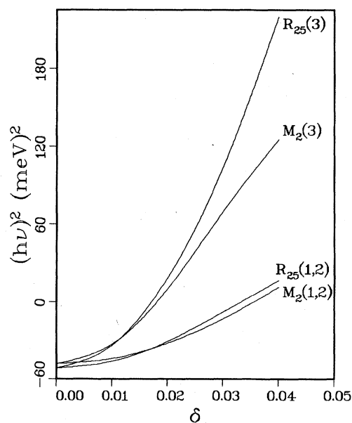
FIG. 9. Plot of the square of the "frequencies" of the low-lying R_{25} and M_2 modes as a function of the low-temperature distortion parameter, \delta , with b = b_0 and f = 1 .
