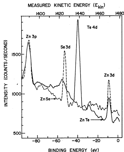
FIG. 2. Electron emission spectrum of ZnSe and ZnTe. The upper scale denotes measured kinetic energy of the electrons, E_{kin} ; lower scale denotes the electron binding energy with reference to the Fermi level of the respective compounds, E_b .
