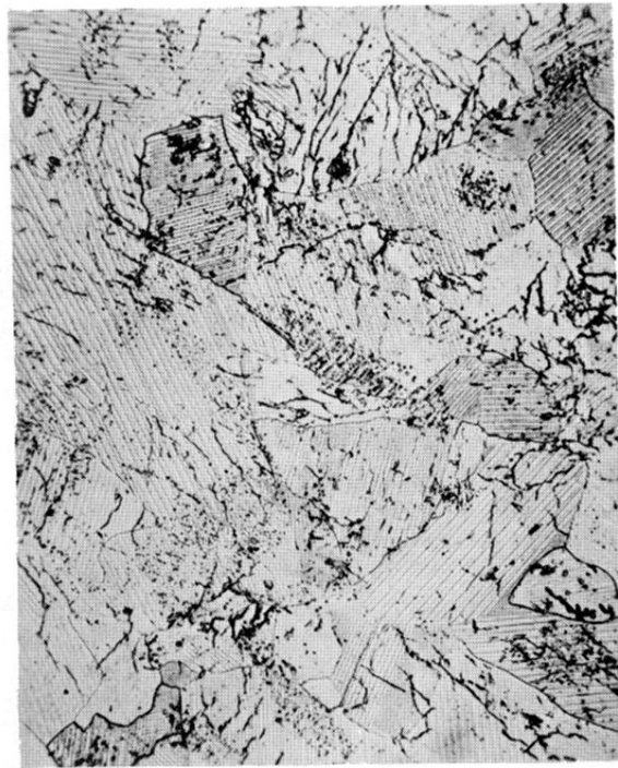
FIG. 1. Bright field photomicrograph of ZrH_{1.81} for a magnification of 250\times .
