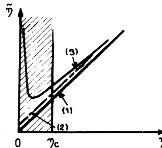
FIG. 4. Schematic representation of the renormalized \eta, \bar{\eta} , as a function of \eta . The renormalization effects are due to the first-order corrections to \Pi . The curve (1) represents the relation \bar{\eta} = \eta . The curve (2) represents \bar{\eta} in the three-dimensional case. The curve (3) represents \bar{\eta} in the two- or one-dimensional case. In the two-dimensional case, \bar{\eta} diverges as |\log \eta| while it diverges as \eta^{-1/2} in the one-dimensional case. The shaded area represents the critical region.
