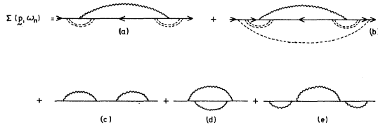
FIG. 2. Diagrammatic representation of the electronic self-energy.
