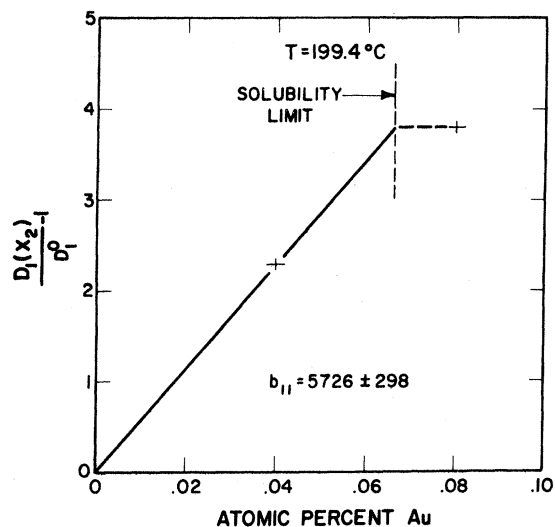
FIG. 4. The enhancement of lead self-diffusivity by additions of gold solute, at 199.4°C. It was ascertained that the addition of 0.08 at. % Au exceeded the solubility limit, and that the solubility limit could be determined from the results as shown in the figure.
