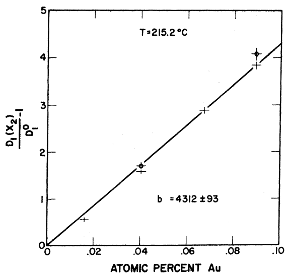
FIG. 5. The enhancement of lead self-diffusivity by additions of gold solute, at 215.2°C. The circled data points were determined from samples which were specially annealed and etched, in lieu of microtoming, prior to deposition of tracer.
