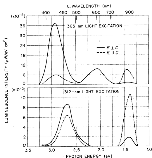
FIG. 3. Emission from neutron-irradiated MgF 2 excited by either 365- or 312-nm light. The solid line depicts data for the electric vector of the emitted light perpendicular to the c axis of the crystal. The dashed line shows data for the electric vector of the emitted light parallel to the crystalline c axis.
