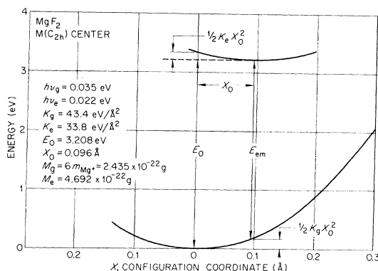
FIG. 5. Configuration-coordinate curve calculated from Eqs. (5)–(7) for the M(C_{2h}) center in MgF_2 .
