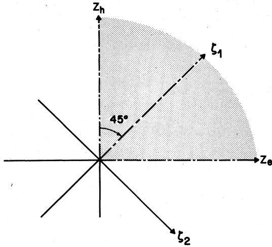
FIG. 1. z_e - z_h plane. Physical interactions occur along the straight-line segments indicated by dash-dot-line, attractive two-body interaction along 45^\circ line and infinitely repulsive one-body forces along horizontal and vertical axes. Wave-function differs from zero only in first quadrant (shaded region). Introduction of potentials along straight-line segments in other quadrants, indicated by solid line, symmetrizes the Hamiltonian without affecting eigenstates
