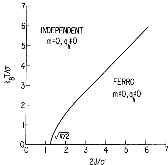
FIG. 1. Phase diagram of an Ising system with infinite-ranged exchange interaction in a random field with Gaussian distribution.
