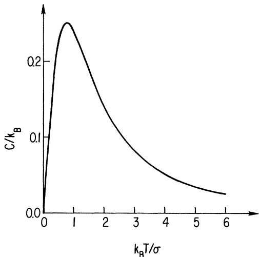
FIG. 2. Temperature dependence of the specific heat in the independent spin phase for 2J/\sigma < (\frac{1}{2}\pi)^{1/2} .
