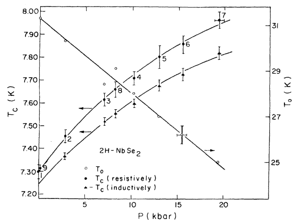
FIG. 1. Pressure dependences of T_0 and T_c of 2H\text{-NbSe}_2 .
