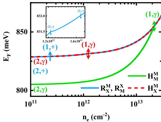
FIG. 10. The Fermi energy in four types of high-symmetric BL MoS 2 , as indicated, as a function of electron density. Here (\nu, \gamma) is the position of E_{c\nu}^\gamma(0) and \uparrow ( \downarrow ) denotes \gamma = + ( - ). The inset shows the E_F around E_{c2}^-(0) and E_{c1}^-(0) in R_M^M and R_X^M stacking BL MoS 2 .
