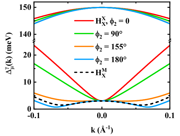
FIG. 5. The energy difference \Delta_\mu^\gamma(k) in H_X^X stacked BL MoS 2 at different \phi_2 , as indicated. The dashed black curve shows \Delta_c^\gamma(k) for H_X^M stacking for comparison. The curves in the upper (lower) part of the panel are the results for the valence (conduction) band.
