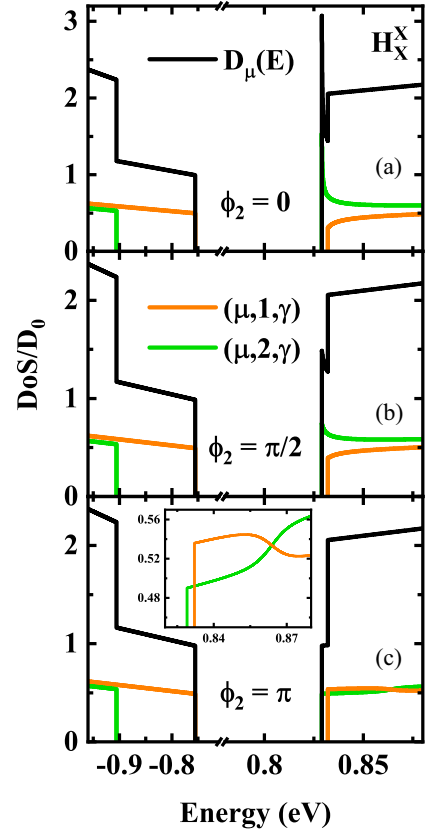
FIG. 8. The electron DoS in H X X stacked BL MoS 2 . ( \mu, \nu, \gamma ) denotes D_{\mu\nu}^{\gamma}(E) . The inset shows the DoS around the conduction band edge.
