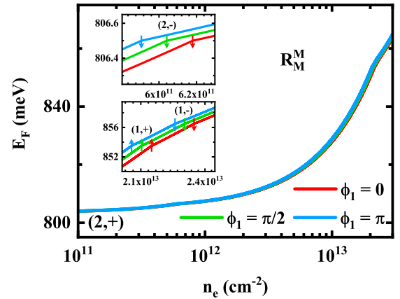
FIG. 12. The Fermi energy in R_M^M stacking BL MoS 2 for different \phi_1 angles as indicated. Here (\nu, \gamma) is the position of E_{c\nu}^\gamma(0) and \uparrow ( \downarrow ) denotes \gamma = + ( - ). The insets are the details of \phi_1 dependence of E_F around E_{c2}^-(0) , E_{c1}^+(0) , and E_{c1}^-(0) .
