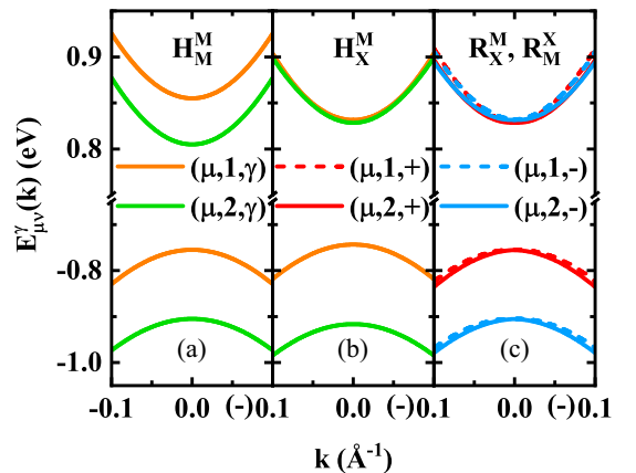
FIG. 2. The electron energy spectra in four types of high-symmetric BL MoS 2 , as indicated. Here (\mu, \nu, \gamma) denotes E_{\mu\nu}^\gamma(k) .
