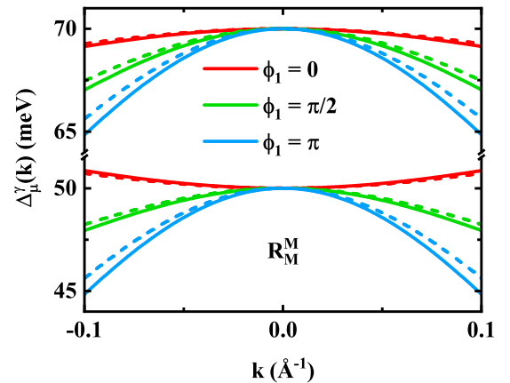
FIG. 6. The energy difference \Delta_\mu^\gamma(k) in R_M^M stacked BL MoS 2 at different \phi_1 , as indicated. The curves in the upper (lower) part of the panel are the results for the valence (conduction) band. The solid/dashed curves denote the spin-up/down states.
