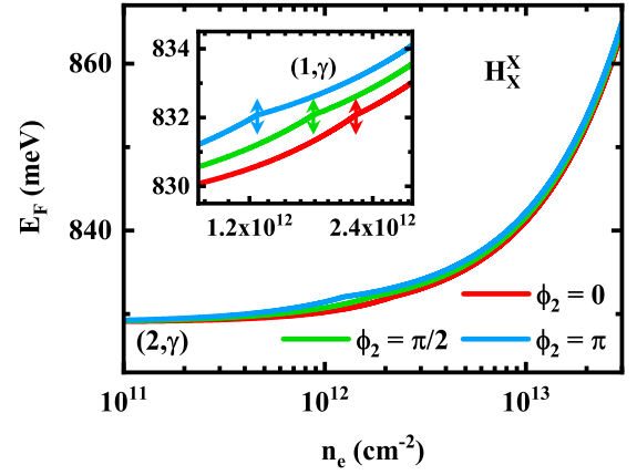
FIG. 11. The Fermi energy in H_X^X stacking BL MoS 2 as a function of electron density for different \phi_2 angles as indicated. (\nu, \gamma) is the position of E_{c\nu}^\gamma(0) and \uparrow ( \downarrow ) denotes \gamma = + ( - ). The inset shows the details of \phi_2 dependence of E_F around E_{c1}^-(0) .
