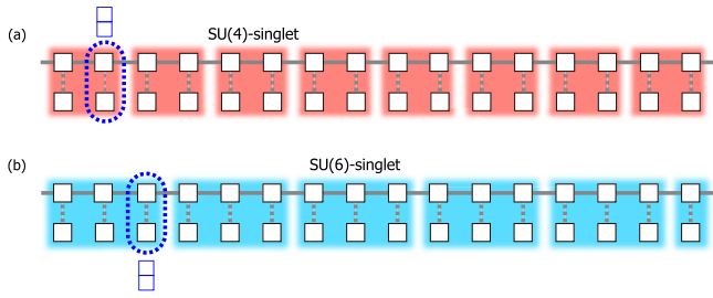
FIG. 4. The insulating ground states ( plaquette phase ) with finite spin gaps formed when J_K > 0 and N = \text{even} : (a) N = 4 and (b) N = 6 . The N spins enclosed by each colored square form an SU(N) singlet. There are N/2 degenerate states related by translation.
