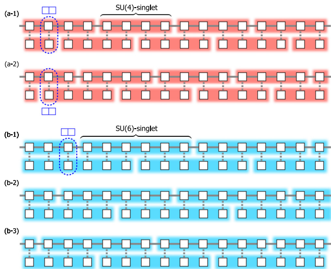
FIG. 5. The N/2 -fold degenerate insulating ground states ( staggered-singlet phase ) with finite spin gaps formed when J_K < 0 and N = \text{even} : (a-1,2) N = 4 and (b-1,2,3) N = 6 . The N spins contained in each colored square form an SU(N) singlet.
