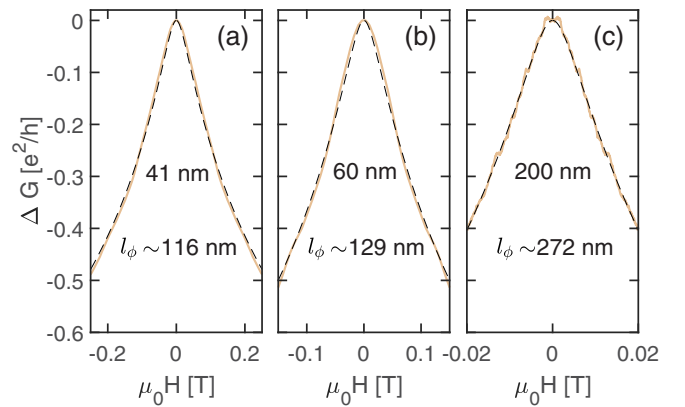
FIG. 3. Field perpendicular WAL magnetoconductance for (a) 41, (b) 60, and (c) 200 nm films. A single band background is subtracted in the 200 nm thick data (SM, Fig. S4). Dashed lines indicate fits to the HLN equation. As the thickness increases, the field range where the WAL is visible decreases, corresponding to an increasing decoherence length.
