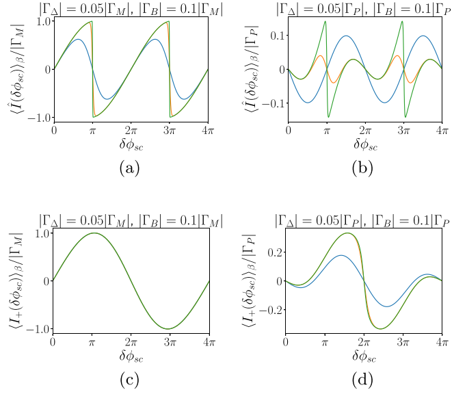
FIG. 4. Thermal average of the current-phase relation with all tunneling terms for different values of \beta for (a) \nu = 1 and (b) \nu = 1/3 . Projected thermal average of the current-phase relation with all tunneling terms for different values of \beta for (c) \nu = 1 and (d) \nu = 1/3 . \beta = 0.01 (blue), 0.1 (orange), and 1 (green) in units of |\Gamma_M|^{-1} in panels (a) and (c) and |\Gamma_P|^{-1} in panels (b) and (d).
