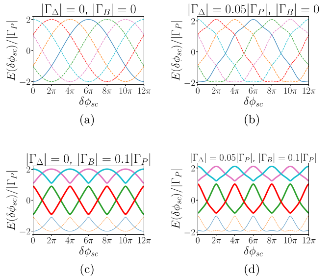
FIG. 2. Spectra of tunneling effective Hamiltonian as functions of the Josephson phase \delta\phi_{sc} with (a) only parafermion tunneling, (b) parafermion and Cooper pair tunneling, (c) parafermion tunneling and backscattering, and (d) backscattering, parafermion, and Cooper pair tunneling. Ground states at each \delta\phi_{sc} are indicated by thin lines. Dashed thin lines can be mapped to solid thin lines by a symmetry transformation. In panels (c) and (d), excited states are indicated with bold lines.
