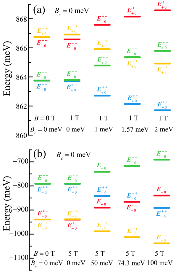
FIG. 3. Schematic illustration of the LLs structure in ML-MoS 2 with LL index n = 0 at the fixed external electrical field strength E_z = 35.25 mV/d for different magnetic fields B , effective Zeeman fields B_c and B_v . The upper panel (a) and lower panel (b) correspond to the conduction and valence bands, respectively.
