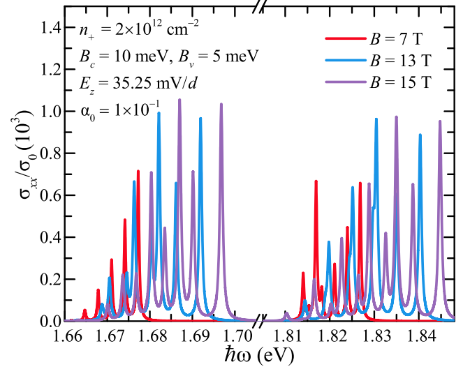
FIG. 10. Magneto-optical conductivity in n -type ML-MoS 2 as a function of radiation photon energy \hbar\omega with including the first six interband electronic transition channels at the fixed electron density n_+ = 2 \times 10^{12} \text{ cm}^{-2} , external electrical field strength E_z = 35.25 \text{ mV/d} , and effective Zeeman fields B_c = 10 \text{ meV} and B_v = 5 \text{ meV} for different magnetic fields B = 7 (red curve), 13 (blue curve), and 15 \text{ T} (purple curve), respectively.
