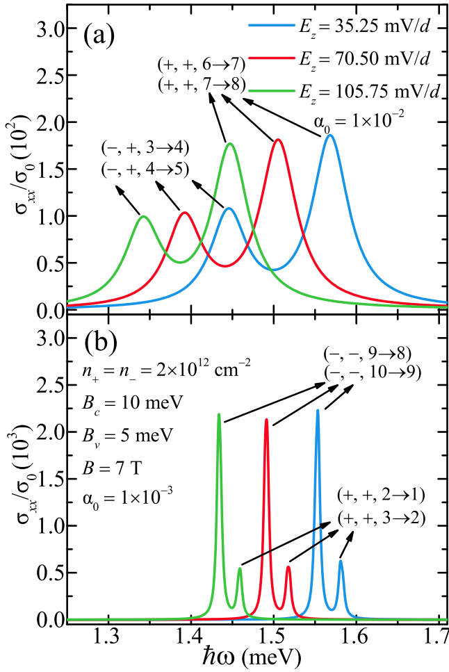
FIG. 7. Magneto-optical conductivity induced by intraband electronic transitions within (a) the conduction band in n -type ML-MoS 2 and (b) the valence band in p -type ML-MoS 2 as a function of radiation photon energy \hbar\omega at the fixed carrier density n_{\beta} = 2.0 \times 10^{12} \text{ cm}^{-2} , effective Zeeman fields B_c = 10 \text{ meV} and B_v = 5 \text{ meV} , and magnetic field B = 7 \text{ T} for different external electrical field strengths E_z = 35.25 \text{ mV/d} (blue curve), E_z = 70.5 \text{ mV/d} (red curve), and E_z = 105.75 \text{ mV/d} (green curve), respectively.
