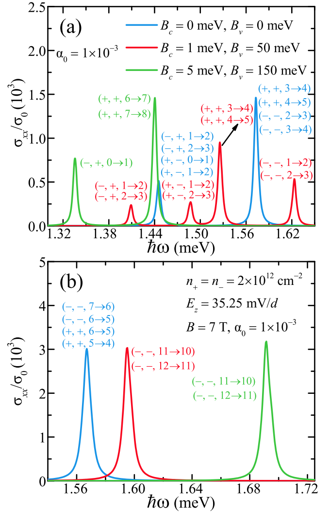
FIG. 6. Magneto-optical conductivity induced by intraband electronic transition within (a) the conduction band and (b) the valence band as a function of radiation photon energy \hbar\omega at the fixed carrier density n_\beta , external electrical field strength E_z = 35.25 \text{ mV/d} and magnetic field B = 7 \text{ T} for different effective Zeeman fields B_c = 0 \text{ meV} , B_v = 0 \text{ meV} (blue curve), B_c = 1 \text{ meV} , B_v = 50 \text{ meV} (red curve), and B_c = 5 \text{ meV} , B_v = 150 \text{ meV} (green curve), respectively.
