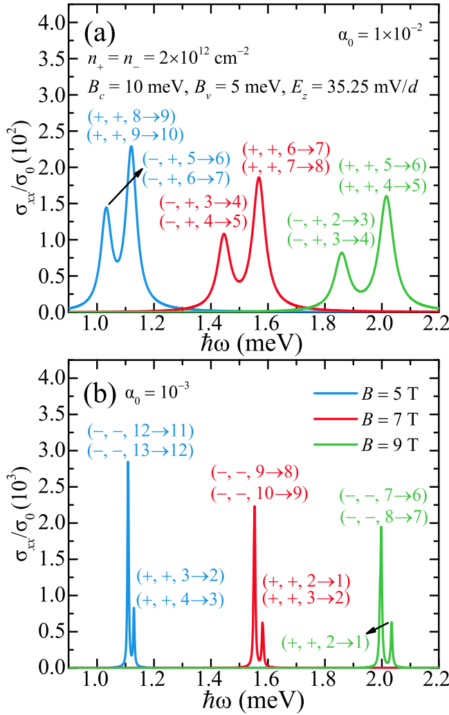
FIG. 5. Magneto-optical conductivity induced via the electronic transition within the conduction bands in (a) and valence bands in (b) in ML-MoS 2 as a function of radiation photon energy \hbar\omega at the fixed carrier densities n_\beta = 2 \times 10^{12} \text{ cm}^{-2} , external electrical field strength E_z = 35.25 \text{ mV/d} , effective Zeeman field factors B_c = 10 \text{ meV} and B_v = 5 \text{ meV} for different magnetic fields B = 5 (blue curve), 7 (red curve), and 9 T (green curve), respectively. The electronic transition channels corresponding to the absorption peaks are indicated by (\zeta, s, n \rightarrow n') . Here \sigma_0 = e^2/h .
