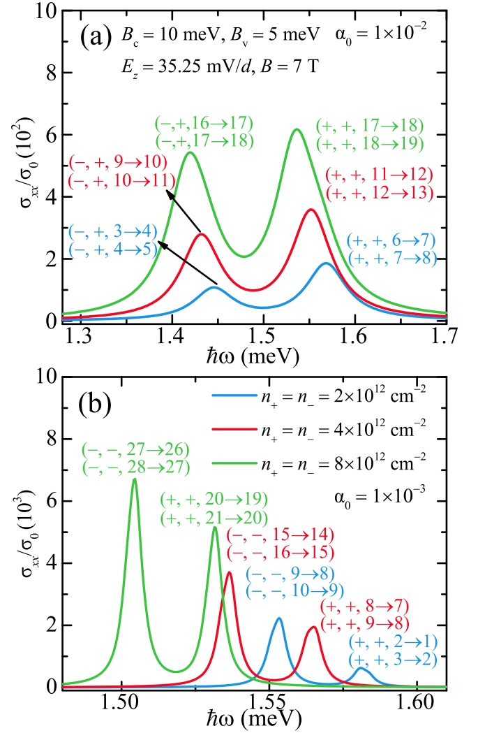
FIG. 8. Magneto-optical conductivity induced by intraband electronic transitions within (a) the conduction band in n -type ML-MoS 2 and (b) the valence band in p -type ML-MoS 2 as a function of radiation photon energy \hbar\omega at the fixed effective Zeeman fields B_c = 10 \text{ meV} and B_v = 5 \text{ meV} , external magnetic field B = 7 \text{ T} and external electrical field strength E_z = 35.25 \text{ mV/d} for different carrier densities n_{\beta} = 2.0 \times 10^{12} \text{ cm}^{-2} (blue curve), n_{\beta} = 4.0 \times 10^{12} \text{ cm}^{-2} (red curve), and n_{\beta} = 8.0 \times 10^{12} \text{ cm}^{-2} (green curve), respectively.
