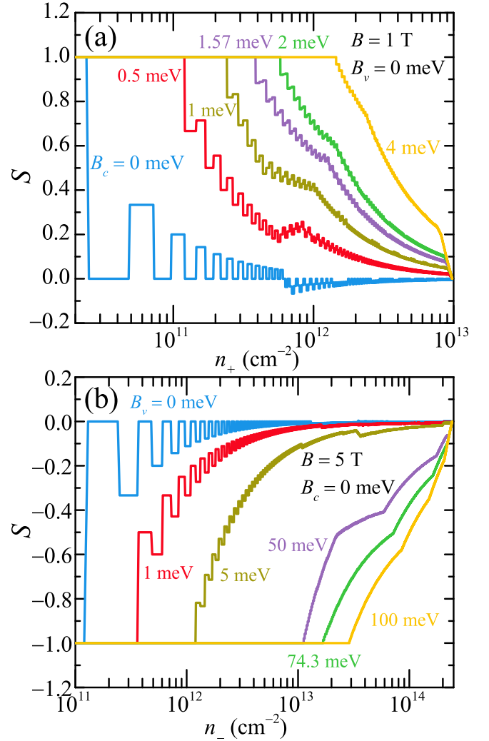
FIG. 4. The spin polarization S of n -type and p -type ML-MoS 2 as a function of electron/hole density n_\beta at the fixed temperature T = 0 K, external electrical field strength E_z = 35.25 mV/d, and magnetic field B for different effective Zeeman fields B_c and B_v . (a) and (b) correspond to the conduction and valence bands, respectively.
