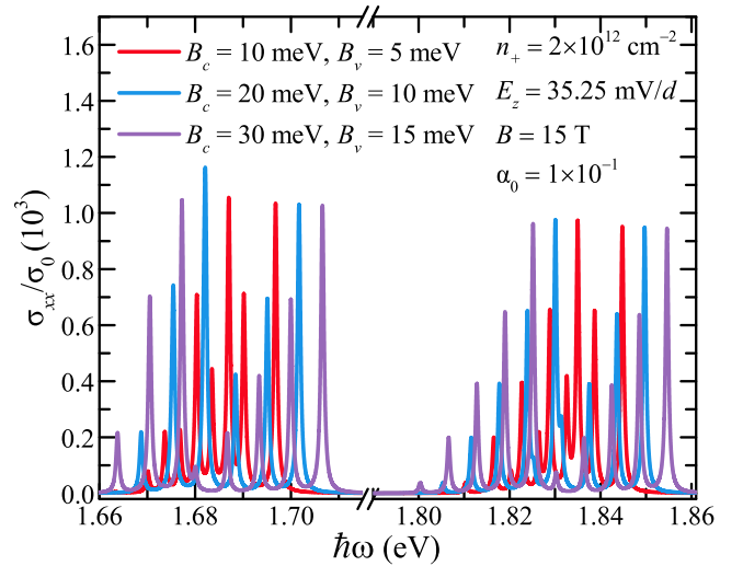
FIG. 11. Magneto-optical conductivity in n -type ML-MoS 2 as a function of radiation photon energy \hbar\omega with including the first six interband electronic transition channels at the fixed electron density n_+ = 2 \times 10^{12} \text{ cm}^{-2} , external electrical field strength E_z = 35.25 \text{ mV/d} and magnetic fields B = 15 \text{ T} for different effective Zeeman fields B_c = 10 \text{ meV} , B_v = 5 \text{ meV} (red curve), B_c = 20 \text{ meV} , B_v = 10 \text{ meV} (blue curve), and B_c = 30 \text{ meV} , B_v = 15 \text{ meV} (purple curve), respectively.
