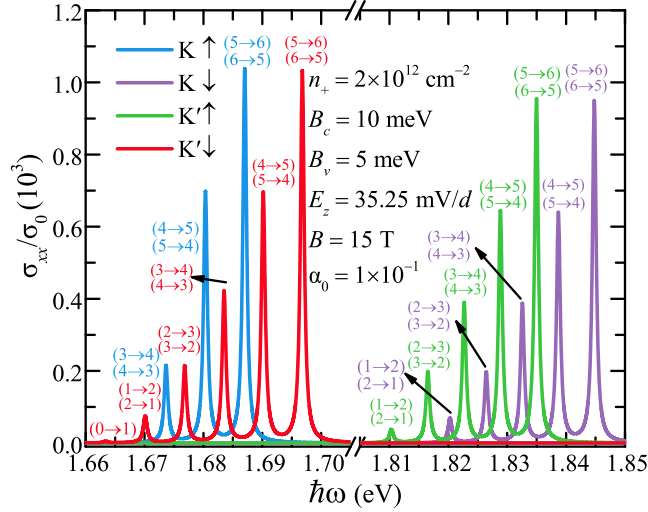
FIG. 9. Magneto-optical conductivity induced by interband electronic transitions from valence band to conduction band in n -type ML-MoS 2 as a function of radiation photon energy \hbar\omega at the fixed electron density n_+ = 2 \times 10^{12} \text{ cm}^{-2} , external electrical field strength E_z = 35.25 \text{ mV/d} , effective Zeeman fields B_c = 10 \text{ meV} and B_v = 5 \text{ meV} , and magnetic field B = 15 \text{ T} . The electronic transition channels corresponding to the absorption peaks are indicated by (\zeta, s, n \rightarrow n') .
