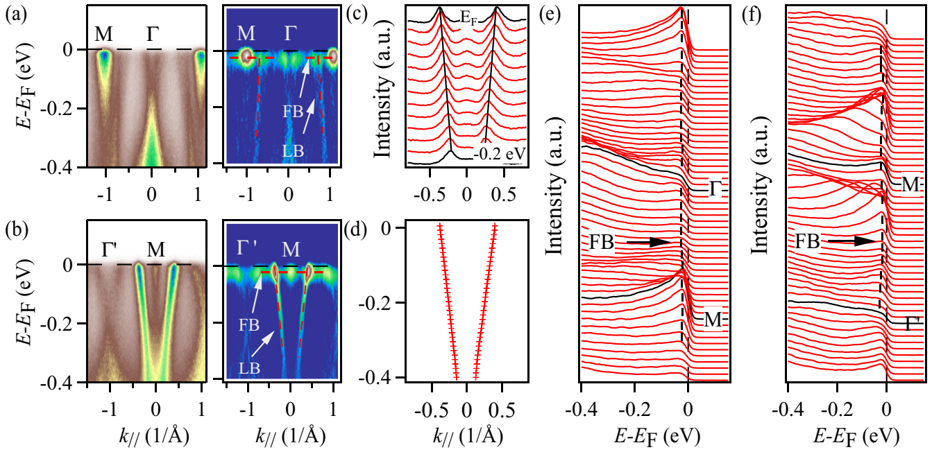
FIG. 3. (a) and (b) Intensity plots and corresponding second derivative plots along the \Gamma - M and \Gamma' - M (perpendicular to \Gamma - M ) directions, respectively. Flat bands (FB) and linear bands (LB) are indicated by the red dashed lines on the corresponding second derivative plots. (c) MDCs of (b) show linear bands. (d) Linear bands abstracted from the fitted MDCs. (e) EDCs of (a). (f) EDCs of (b). The black dashed lines are guides to flat bands.
