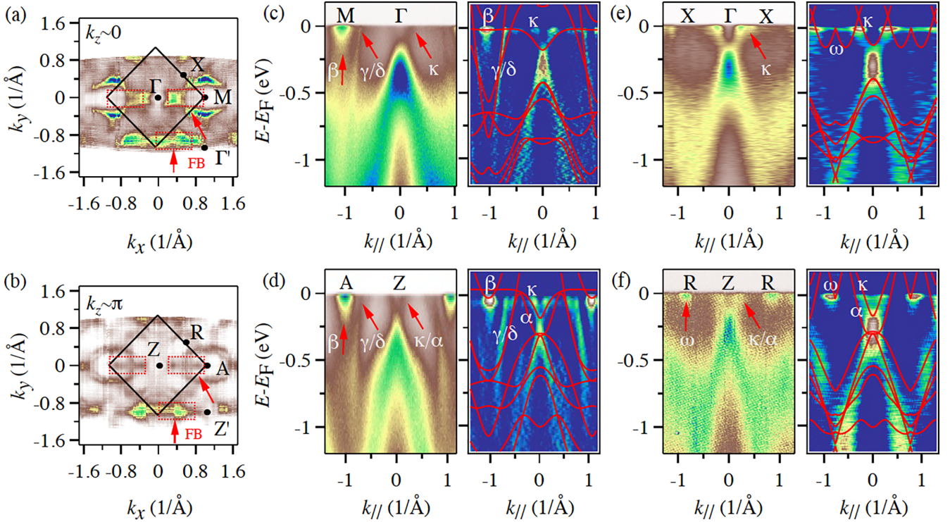
FIG. 1. (a) and (b) Integrated intensity plots at E_F \pm 10 meV taken on the k_z \sim 0 ( \Gamma - X - M ) and k_z \sim \pi ( Z - R - A ) plane, respectively. The black solid lines indicate the two-dimensional BZ projected on the (001) surface. The red frames indicated by the arrow lines show shadowy FSs formed by the flat band. (c) and (d) Intensity plots and corresponding second derivative plots along the \Gamma - M and Z - A directions, respectively. (e) and (f) The same as (c) and (d), but along the \Gamma - X and Z - R directions, respectively. The bands near E_F are indicated by the red arrow lines on the intensity plots and are marked on the corresponding second derivative plots. The red solid lines on the corresponding second derivative plots are DFT-calculated bands renormalized by a factor of 1.4.
