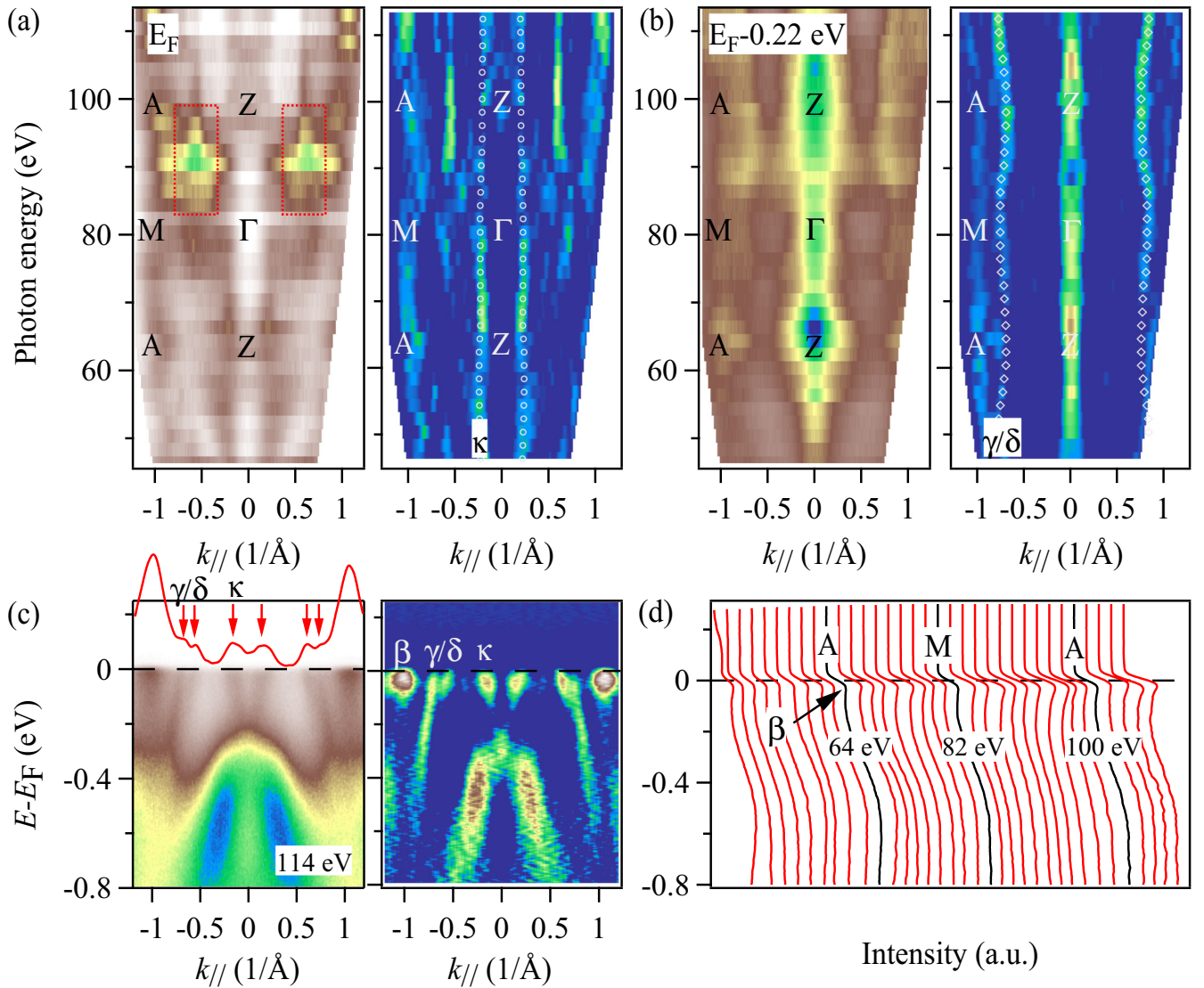
FIG. 2. (a) and (b) Integrated intensity plots ( \pm 10 meV) and corresponding second derivative plots on the k_{//} - k_z plane taken at E_F and E_F - 0.22 eV, respectively. Photon energies used for the k_z dispersion measurement were from 46 to 114 eV. High-symmetry points and the band names are indicated. The shadows from the flat bands indicated by the red frames in the integrated intensity plots are enhanced from around 84 to 98 eV due to the matrix element effects. (c) Intensity plot and corresponding second derivative plot along the \Gamma -M direction taken by photon energy of 114 eV ( k_z \sim \pi/2 ). The appended red solid curve is MDC at E_F . The peaks indicated by the red arrows are the band-crossing point at E_F . (d) EDCs along the A-M-A direction.
