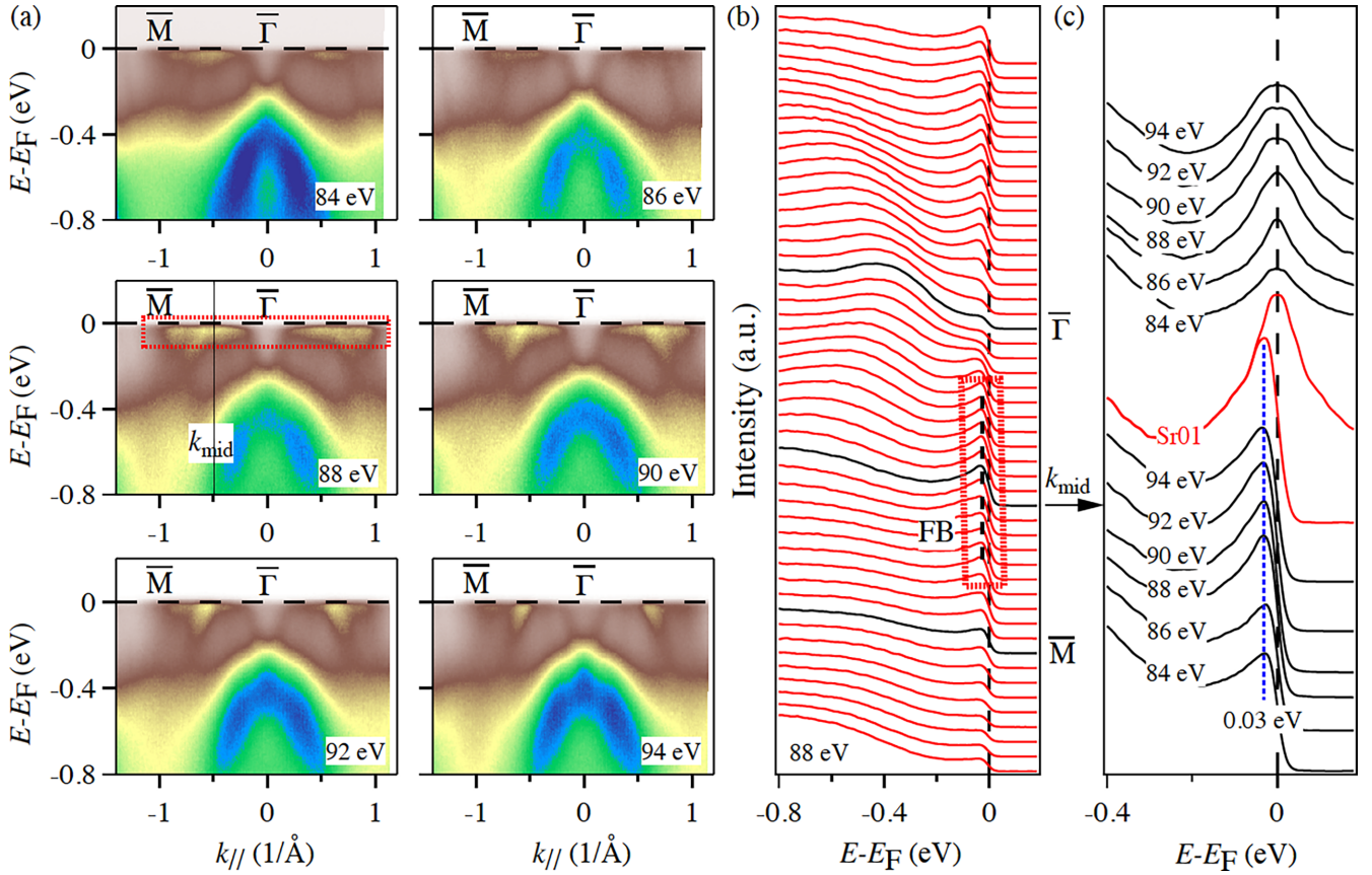
FIG. 4. (a) Intensity plots along the \bar{\Gamma} - \bar{M} direction taken by photon energies of 84, 86, 88, 90, 92, and 94 eV, respectively, as noted in the individual panels. The red frame in one panel of 88 eV, as a representative, indicates the flat bands along \bar{\Gamma} - \bar{M} in all panels and the k_{mid} is in the middle of \bar{\Gamma} - \bar{M} . (b) EDCs of the intensity plot taken with 88-eV photons in (a). The red frame indicates the flat band along \bar{\Gamma} - \bar{M} . (c) Black curves are the EDCs and symmetrized EDCs at k_{mid} . The red curves are the corresponding EDC and symmetrized EDC of Sr(Co 0.9 Ni 0.1 ) 2 As 2 [25]. Symmetrization allows us to approximately remove the effect of the Fermi-Dirac function at k_F .
