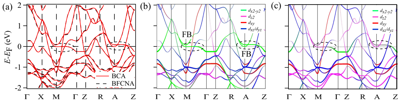
FIG. 5. (a) DFT calculation with spin-orbit coupling (SOC) along high-symmetry directions. Flat bands are indicated by the black ellipses. The experimental crystal structures (space group 14/mmm, No. 139) of BaCo 2 As 2 (red solid lines) with lattice constants a = 3.9537 \text{ \AA} , c = 12.6524 \text{ \AA} , and z_{As} = 1.278 \text{ \AA} [34] and Ba(Fe 1/3 Co 1/3 Ni 1/3 ) 2 As 2 (black dashed lines) with lattice constants a = 3.9920 \text{ \AA} , c = 12.6191 \text{ \AA} , and z_{As} = 1.282 \text{ \AA} [28] were used in the calculations. (b) and (c) DFT calculation with SOC and 3d orbital projections along high-symmetry directions. d_{x2-y2} (green) orbital is mainly shown in (e), and d_{z2} (magenta) orbital is mainly shown in (f).
