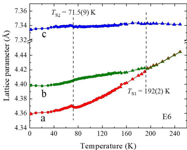
FIG. 2. Temperature dependence of lattice parameters refined from E6 data, assuming I4/mmm and I4/mmm space groups at high and low temperature, respectively.
