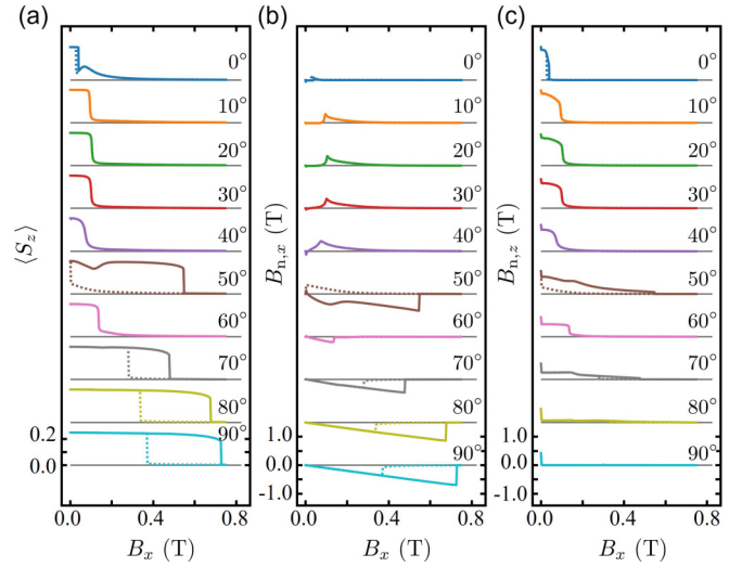
FIG. 9. The computed results of \langle S_z \rangle (a), B_{n,x} (b), and B_{n,z} (c) in the steady state of the system under various values of the polar angle \theta_Q of the NQI major principal axis. Solid and dashed lines denote the results for increasing and decreasing B_x , respectively. All nuclei are assumed to have a spin of 3/2 , for simplicity.
