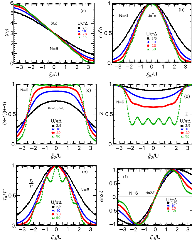
FIG. 3. Fermi-liquid parameters of an SU(6) dot are plotted as a function of \xi_d/U for U/(\pi\Delta) = 2/5, 1.0, 2.0, 5.0 . (a) \langle n_d \rangle , (b) \sin^2 \delta , (c) rescaled Wilson ratio \tilde{K} \equiv (N-1)(R-1) , (d) renormalized factor z , (e) T_K/T^* , and (f) \sin 2\delta . Here T_K is defined as the value of T^* \equiv 1/(4\chi_{\sigma\sigma}) at half filling \xi_d = 0 .
