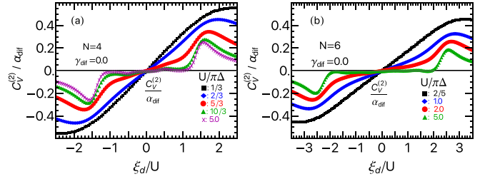
FIG. 6. Effects of bias-voltage asymmetry \alpha_{\text{dif}} on order (eV)^2 nonlinear current: C_V^{(2)}/\alpha_{\text{dif}} given by Eq. (4.4) for symmetric junctions with \gamma_{\text{dif}} = 0.0 is plotted vs \xi_d/U , varying interactions from weak to strong. (a) For SU(4) quantum dots with U/(\pi\Delta) = 1/3, 2/3, 5/3, 10/3, 5.0 . (b) For SU(6) quantum dots with U/(\pi\Delta) = 2/5, 1.0, 2.0, 5.0 .
