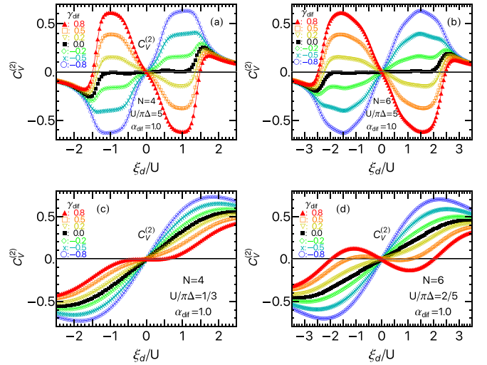
FIG. 8. C_V^{(2)} for a large bias-voltage asymmetry \alpha_{\text{dif}} = 1.0 is plotted vs \xi_d , varying tunnel asymmetries, as \gamma_{\text{dif}} = -0.8 ( \circ ), -0.5 ( \times ), -0.2 ( \diamond ), 0.0 ( \blacksquare ), 0.2 ( \nabla ), 0.5 ( \square ), and 0.8 ( \triangle ). (Left panels) For SU(4) quantum dots and (right panels) for SU(6) ones, with (top panels) a strong interaction U/(\pi\Delta) = 5.0 and (bottom panels) weak interactions U/(\pi\Delta) = 1/3 for SU(4) and U/(\pi\Delta) = 2/5 for SU(6).
