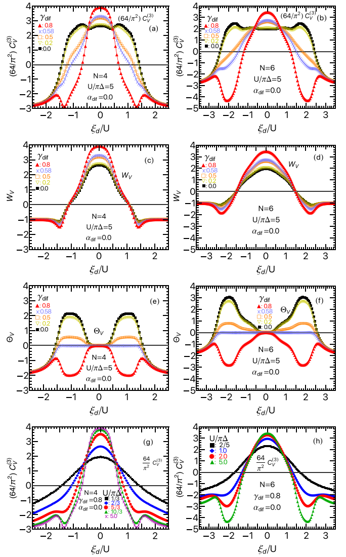
FIG. 10. Effects of tunnel asymmetry \gamma_{\text{dif}} on order (eV)^3 non-linear current: (top panels) C_V^{(3)} and the components (upper middle panels) W_V and (lower middle panels) \Theta_V defined in Eqs. (5.6) and (5.7) for symmetrical bias voltages \alpha_{\text{dif}} = 0.0 are plotted vs \xi_d/U , varying tunnel asymmetries, as for \gamma_{\text{dif}} = 0.0 (■), 0.2 (▽), 0.5 (□), 0.58 (×), 0.8 (△). Interaction strength is chosen to be U/(\pi\Delta) = 5.0 for (a)–(f): (left panels) for SU(4) quantum dots and (right panels) for SU(6) quantum dots. (Bottom panels) U dependence of C_V^{(3)} , calculated for a fixed large tunnel asymmetry \gamma_{\text{dif}} = 0.8 , (g) U/(\pi\Delta) = 1/3 (■), 2/3 (◇), 5/3 (○), 10/3 (△), 5.0 (×) for SU(4) and (h) U/(\pi\Delta) = 2/5 (■), 1.0 (◇), 2.0 (○), 5.0 (△) for SU(6).
