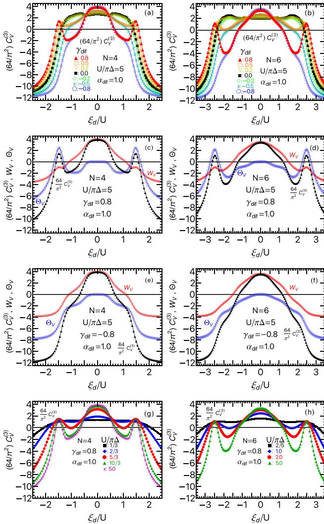
FIG. 12. Behavior of C_V^{(3)} at large bias asymmetry \alpha_{\text{dif}} = 1 is plotted vs \xi_d for (left panels) SU(4) and (right panels) SU(6) quantum dots. Top panels: Tunnel asymmetry is varied as \gamma_{\text{dif}} = -0.8 ( \circ ), -0.5 ( \times ), -0.2 ( \diamond ), 0.0 ( \blacksquare ), 0.2 ( \nabla ), 0.5 ( \square ), and 0.8 ( \triangle ). In addition, two-body part W_V ( \square ) and three-body part \Theta_V ( \circ ) are plotted together with C_V^{(3)} ( \blacktriangle ) for two large opposite tunnel asymmetries: (upper middle panels) \gamma_{\text{dif}} = 0.8 , and (lower middle panels) \gamma_{\text{dif}} = -0.8 . Interaction strength is chosen to be U/(\pi\Delta) = 5.0 in (a)–(f). Bottom panels show the U dependence of C_V^{(3)} for \gamma_{\text{dif}} = 0.8 : (g) U/(\pi\Delta) = 1/3, 2/3, 5/3, 10/3, 5.0 for SU(4) and (h) U/(\pi\Delta) = 2/5, 1.0, 2.0, 5.0 for SU(6).
