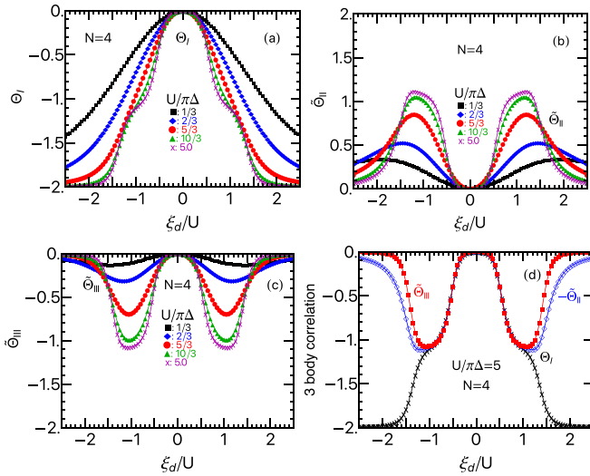
FIG. 2. Three-body correlation functions of an SU(4) dot plotted vs \xi_d/U for U/\pi\Delta = 1/3, 2/3, 5/3, 10/3, 5.0 : (a) \Theta_I , (b) \Theta_{II} , and (c) \Theta_{III} . (d) Comparison of \Theta_I , -\Theta_{II} , and \Theta_{III} at a large interaction U/(\pi\Delta) = 5.0 . It indicates that \Theta_I \simeq -\Theta_{II} \simeq \Theta_{III} over a wide range of -U \lesssim \xi_d \lesssim U .
