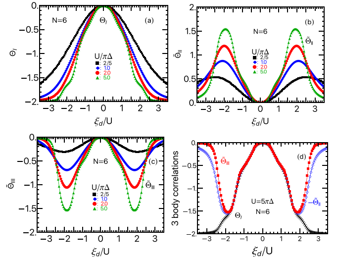
FIG. 4. Three-body correlation functions of an SU(6) dot plotted vs \xi_d/U for U/\pi\Delta = 2/5, 1.0, 2.0, 5.0 : (a) \Theta_I , (b) \Theta_{II} , and (c) \Theta_{III} . (d) Comparison of \Theta_I, -\Theta_{II}, and \tilde{\Theta}_{III} at a large interaction U/(\pi\Delta) = 5.0 . It indicates that \Theta_I \simeq -\Theta_{II} \simeq \tilde{\Theta}_{III} over a wide range of -(N-1)U/2 \lesssim \xi_d \lesssim (N-1)U/2 for N = 6 .
