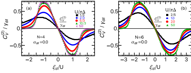
FIG. 5. Effects of tunnel asymmetry \gamma_{\text{dif}} on order (eV)^2 nonlinear current: C_V^{(2)}/\gamma_{\text{dif}} given by Eq. (4.3) for symmetrical bias voltages \alpha_{\text{dif}} = 0.0 is plotted vs \xi_d/U , varying interactions from weak to strong. (a) For SU(4) quantum dots with U/(\pi\Delta) = 1/3, 2/3, 5/3, 10/3, 5.0 . (b) For SU(6) quantum dots with U/(\pi\Delta) = 2/5, 1.0, 2.0, 5.0 .
