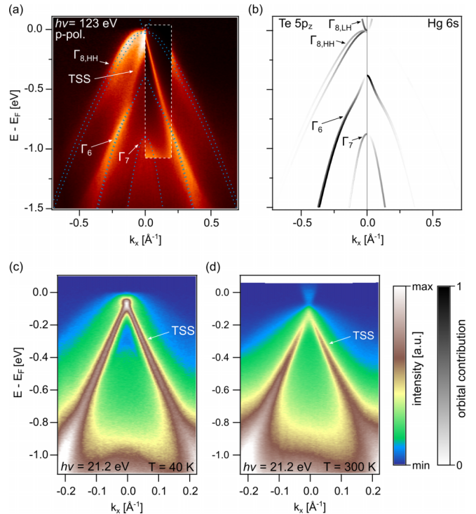
FIG. 4. (a) ARPES data near the \Gamma point taken with h\nu = 123 eV and p -polarized light. The inset shows ARPES data obtained with He I_\alpha line ( h\nu = 21.2 eV) for which the cross section of the topological surface state is much larger than for the bulk bands. (b) Calculated bulk band structure projected on Te 5p_z and Hg 6s orbitals. (c) and (d) ARPES datasets measured at (b) T = 40 K and (c) 300 K ( h\nu = 21.2 eV).
