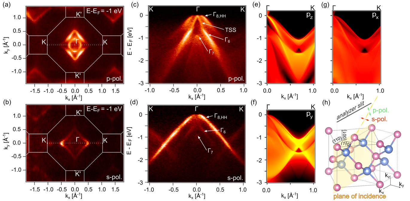
FIG. 3. (a) and (b) Constant-energy ARPES datasets obtained with p - and s -polarized light. The boundaries of the bulk BZ are indicated. (c) and (d) ARPES data along the K - \Gamma - K direction for p - and s -polarized light. (e)–(g) Calculations of the (001)-projected surface spectral function along \Gamma K projected on different Te 5p orbitals. (h) Schematic of the experimental geometry. The datasets in all panels were taken with h\nu = 123 eV.
