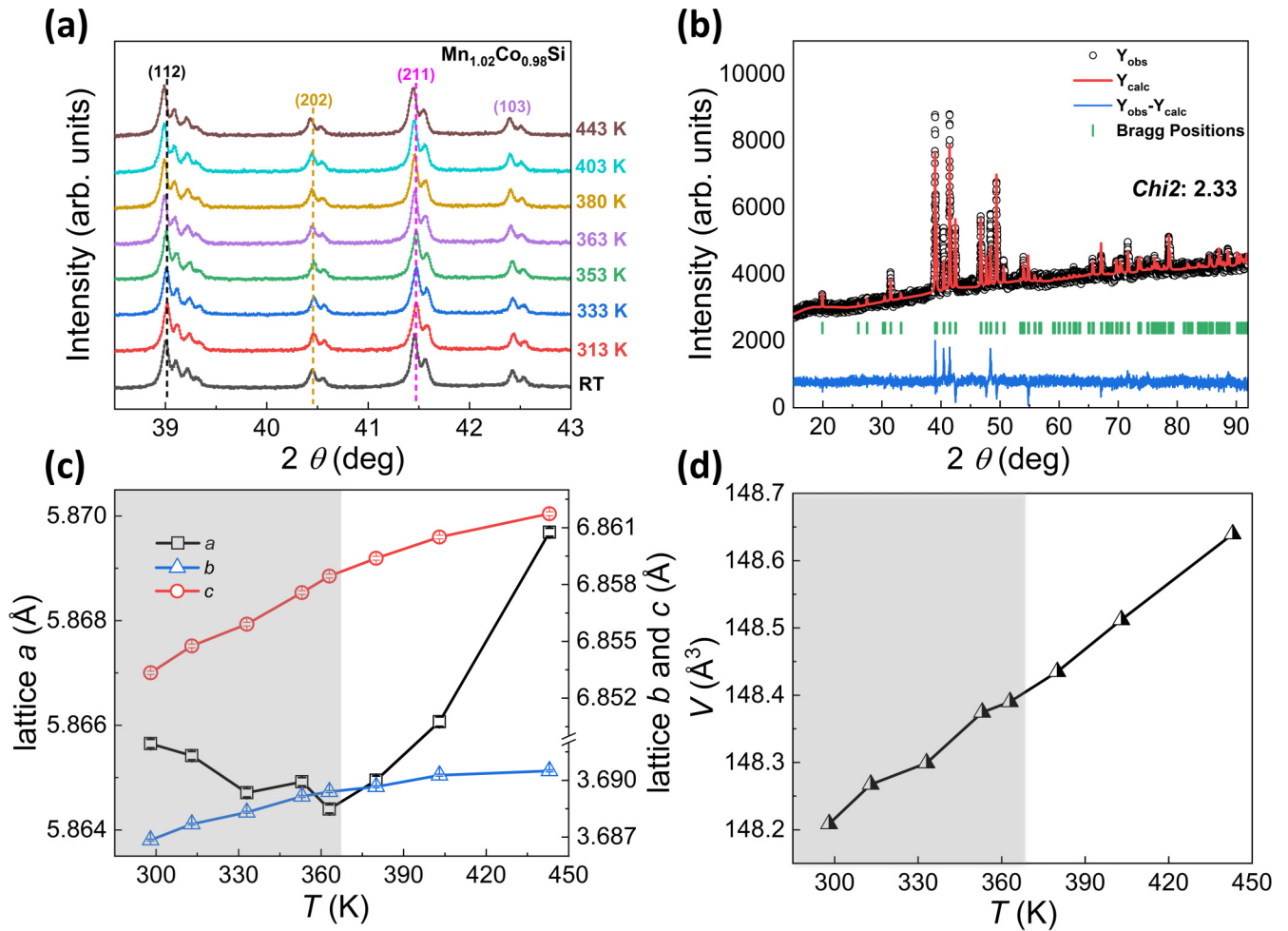
FIG. 1. (a) XRD patterns for the orthorhombic Mn 1.02 Co 0.98 Si compound measured at different temperatures. (b) Rietveld refinement of the XRD pattern at 313 K. (c) Derived lattice parameters and (d) unit-cell volume as a function of the temperature for the Mn 1.02 Co 0.98 Si compound.
