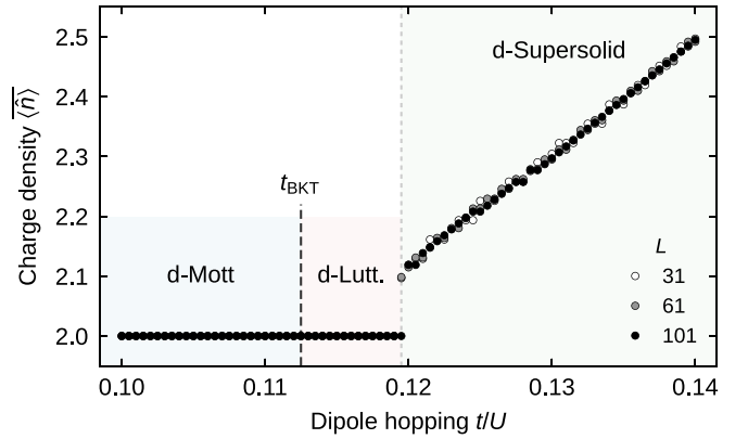
FIG. 8. Transition to incommensurable densities. Average charge density \langle \hat{n} \rangle for a cut through the grand-canonical phase diagram along the line of fixed chemical potential \mu/U = 0.95 . Different unit-cell sizes L used in the iDMRG simulations are compared. We observe an apparent first-order transition into a compressible state with continuously varying charge density.
