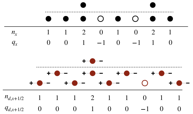
FIG. 2. Microscopic dipole density. Mapping between product states in the boson occupation number basis (upper panel) and microscopic dipole occupation numbers on the bonds of the lattice (lower panel). Here, n_x and n_{d,x+1/2} are non-negative, whereas q_x and q_{d,x+1/2} are defined with respect to the average densities (dashed line). For a state at integer boson filling within the same dipole moment sector as the uniform state |n\rangle , the resulting dipole model exhibits integer filling as well. See main text for a detailed description of the mapping.
