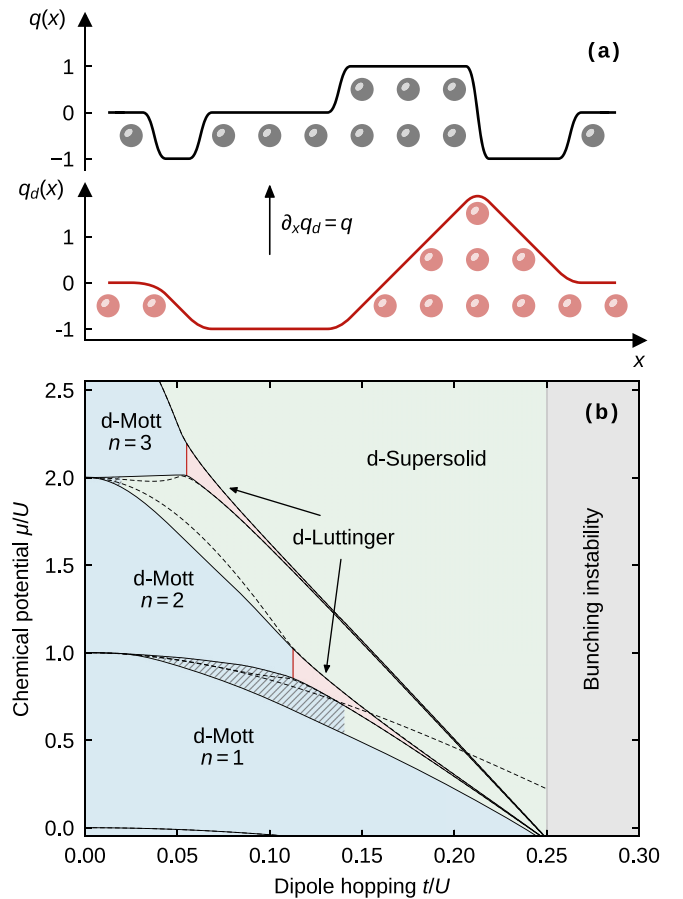
FIG. 1. Fractonic phases of matter in one dimension. (a) At low energies, area-law fluctuations of the charge q(x) permit the definition of a local dipole density q_d(x) as \partial_x q_d(x) = q(x) . This allows us to apply bosonization to construct a low-energy effective field theory for microscopic dipoles, which are composites of fractons. (b) The grand-canonical phase diagram of the dipole-conserving Bose-Hubbard model features three distinct phases: an incompressible dipole Mott insulator (d-Mott), shown in blue, within lobes of integer filling; an incompressible dipole condensate in form of a Luttinger liquid of dipoles (d-Luttinger), located in the red region at the tips of lobes, which extends to the bunching instability (grey region); and a compressible supersolid of dipoles (d-Supersolid) at noninteger filling in the green region. Solid black lines correspond to estimated phase boundaries from grand-canonical iDMRG computations. The dashed black lines indicate the energies for adding or removing a single particle (see text below). The regions between the Mott lobes at small dipole hopping t/U (hatched region) additionally host a Mott insulating phase at noninteger filling, which for instance at n = 3/2 is stable up to t/U \approx 0.14 .
