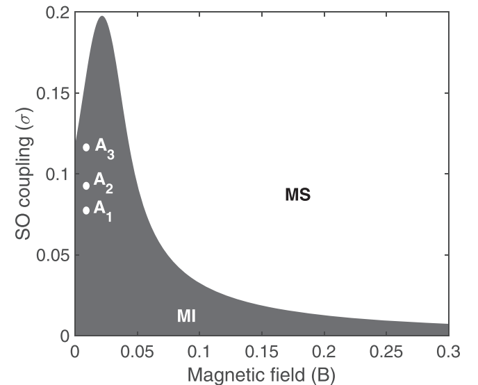
FIG. 11. The panels show the numerically generated phase diagrams in the (B, \sigma) plane for I_1 = I_2 = 3 . The wave number K_1 = K_2 = 0.75 , and the initial densities n_0 = 1 , while the other parameter values are G = 1.1 , g = 3.64 , \tilde{g} = -0.364 , \Gamma = 3 , and h = -0.1 . The points A_1 , A_2 , and A_3 correspond to values of B and \sigma that were used to generate Fig. 12. MI indicates the region of instability, and MS (modulational stability) indicates the region of stability.
