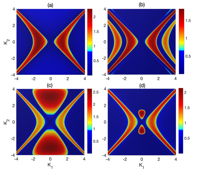
FIG. 1. The panels show the variation of the MI gain \zeta(\Omega) in the (K_1, K_2) plane for (a) \sigma = 0.03 , (b) \sigma = 0.5 , (c) \sigma = 0.7 , and (d) \sigma = 0.9 , with the other parameters being I = 3.0 , G = 1.1 , g = 3.64 , \tilde{g} = -0.364 , h = -0.1 , and n_{10} = n_{20} = n_0 = 1 .
