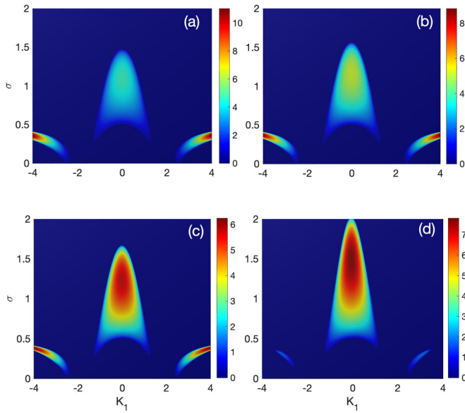
FIG. 2. The panels show the variation of the MI gain \zeta(\Omega) versus the perturbation wave number K_1 and the photonic SO coupling strength \sigma for (a) I_1 = I_2 = 1 , (b) I = 3 , (c) I_1 = I_2 = 5 , and (d) I_1 = I_2 = 6 , with K_2 = 1.5 , G = 1.1 , g = 3.64 , \tilde{g} = -0.364 , h = -0.1 , and n_{10} = n_{20} = n_0 = 1 .
