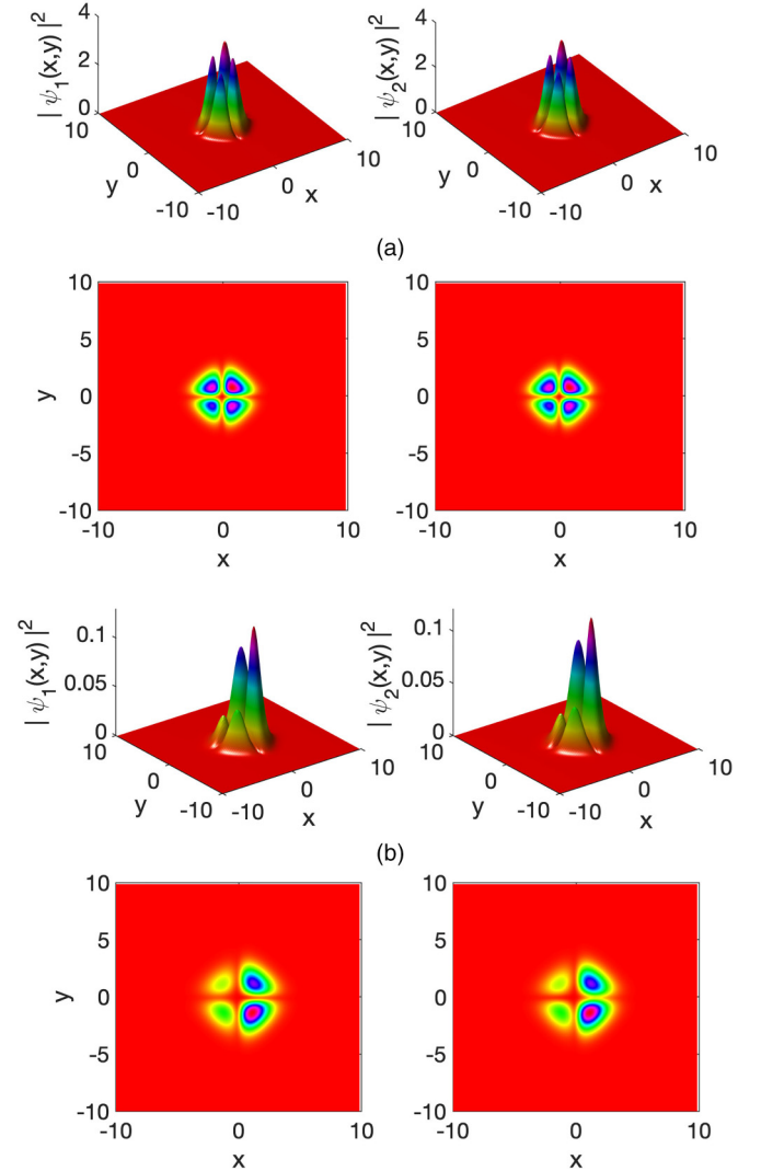
FIG. 8. Development of MI, with (a) and (b) showing |\psi_1|^2 and |\psi_2|^2 , and their corresponding density plots obtained from numerical simulations using the points A_3 and A_4 of the phase diagram of Fig. 7. The other parameter values are G = 1.1 , g = 3.64 , \tilde{g} = -0.364 , K_1 = K_2 = 2 , \Gamma = 3 , h = -0.1 , and n_{10} = n_{20} = n_0 = 1 . The left column corresponds to |\psi_1|^2 , and the right column to |\psi_2|^2 .
