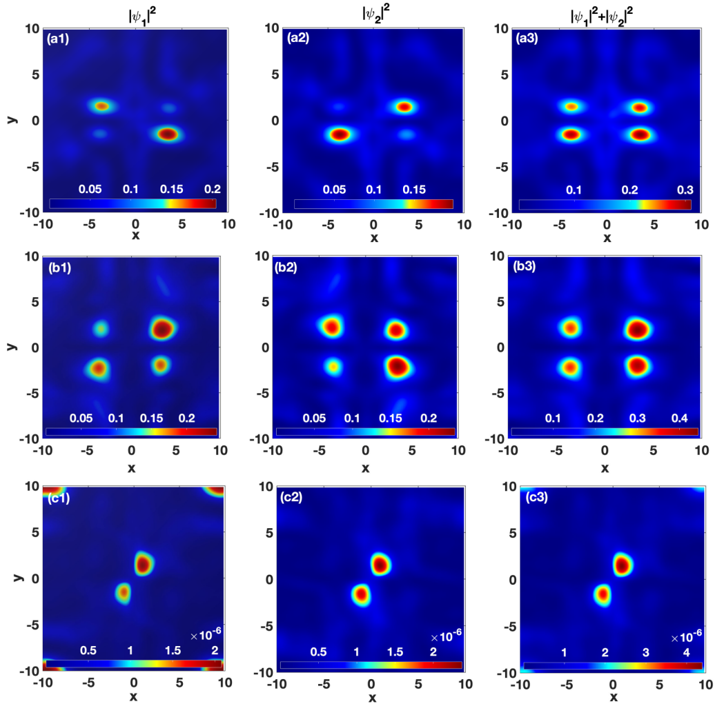
FIG. 6. Development of MI, with (aj) j=1,2,3 , (bj) j=1,2,3 , and (cj) j=1,2,3 corresponding, respectively, to \sigma = 0.009 , \sigma = 0.018 , \sigma = 0.024 and the other parameters being I_1 = I_2 = 2 , G = 1.1 , g = 3.64 , \tilde{g} = -0.364 , K_1 = K_2 = 2 , \Gamma = 3 , h = -0.1 , n_{10} = n_{20} = n_0 = 1 , and B = 0.02 . From left to right, the columns correspond to |\psi_1|^2 , |\psi_2|^2 , and (|\psi_1|^2 + |\psi_2|^2) .
