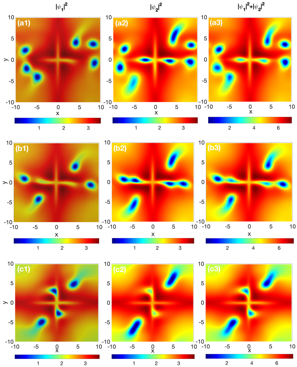
FIG. 12. Development of MI, with (aj) j=1,2,3 , (bj) j=1,2,3 , and (cj) j=1,2,3 corresponding, respectively, to \sigma = 0.75 , \sigma = 0.9 , \sigma = 0.12 and the other parameter values being I_1 = I_2 = 2 , G = 1.1 , g = 3.64 , \tilde{g} = -0.364 , K_1 = K_2 = 0.75 , \Gamma = 3 , h = -0.1 , n_{10} = n_{20} = n_0 = 1 , and B = 0.01 . From left to right, the columns correspond to |\psi_1|^2 , |\psi_2|^2 , and (|\psi_1|^2 + |\psi_2|^2) .
