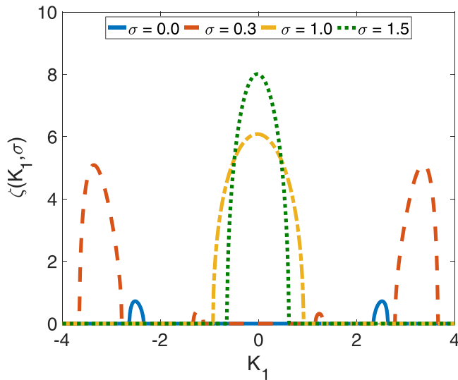
FIG. 3. The panel shows the cross section of the MI growth rate \zeta(\Omega) versus the perturbation wave number K_1 for K_2 = 1.5 . This corresponds to the results of Fig. 2(c), with the lines corresponding to increasing values of the photonic SO coupling strength \sigma . The rest of the parameter values are I_1 = I_2 = 5 , G = 1.1 , g = 3.64 , \tilde{g} = -0.364 , h = -0.1 , and n_{10} = n_{20} = n_0 = 1 .
