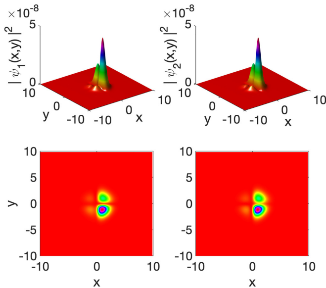
FIG. 9. Development of MI using values of \sigma and B from the point A_5 of the phase diagram of Fig. 7. The left column corresponds to |\psi_1|^2 , and the right column to |\psi_2|^2 , along with their corresponding density plots. The other parameter values are G = 1.1 , g = 3.64 , \tilde{g} = -0.364 , K_1 = K_2 = 2 , \Gamma = 3 , h = -0.1 , and n_{10} = n_{20} = n_0 = 1 .
