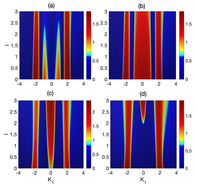
FIG. 5. The panels show the distribution of the MI gain \zeta(\Omega) versus the perturbation wave number K_1 and the input power I = I_1 = I_2 for (a) \sigma = 0.03 , (b) \sigma = 0.5 , (c) \sigma = 0.7 , and (d) \sigma = 0.9 , with the other parameters being K_2 = 1.5 , G = 1.1 , g = 3.64 , \tilde{g} = -0.364 , \Gamma = 3 , h = -0.1 , and n_{10} = n_{20} = n_0 = 1 .
