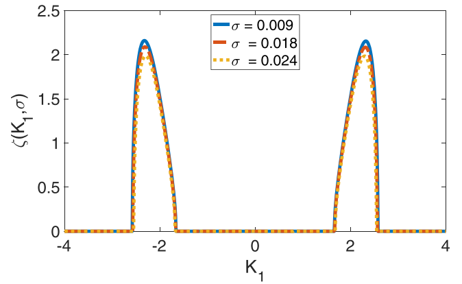
FIG. 4. The panels show the variation of the MI gain \zeta(\Omega) versus the wave number K_1 under the effect of weak values of the photonic SO coupling for K_2 = 2 and the parameter values I = 3.0 , G = 1.1 , g = 3.64 , \tilde{g} = -0.364 , h = -0.1 , and n_{10} = n_{20} = n_0 = 1 .
