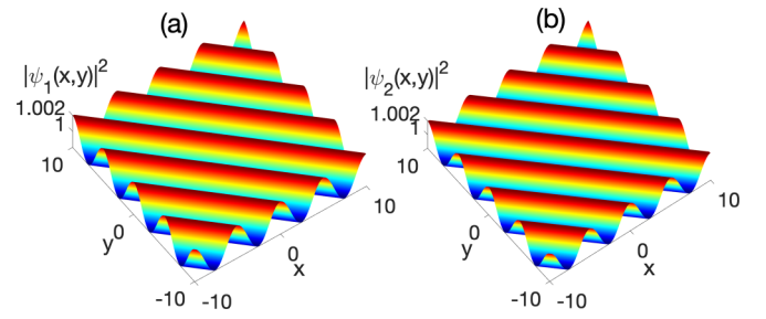
FIG. 10. Example of modulational stability (MS) resulting from the point C_0 of the phase diagram of Fig. 7, (a) and (b) showing |\psi_1|^2 and |\psi_2|^2 . The other parameter values are G = 1.1 , g = 3.64 , \tilde{g} = -0.364 , K_1 = K_2 = 2 , \Gamma = 3 , h = -0.1 , and n_{10} = n_{20} = n_0 = 1 . The left column corresponds to |\psi_1|^2 , and the right column to |\psi_2|^2 .
