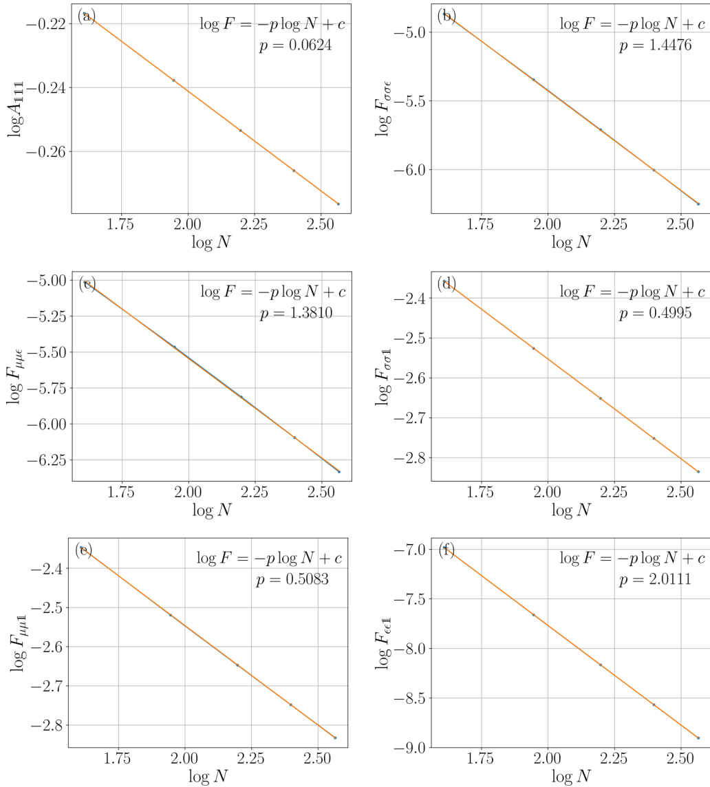
FIG. 10. (a) Scaling of A_{111} , computed for N_1 = 2N , N_2 = 2N , and N_3 = 4N . [(b)–(f)] Scaling of F_{\alpha\beta\gamma} , where A_{\alpha\beta\gamma} is computed for N_1 = 2N + 1 , N_2 = 2N - 1 , and N_3 = 4N . To simulate small system, N takes value from 5 to 12.
