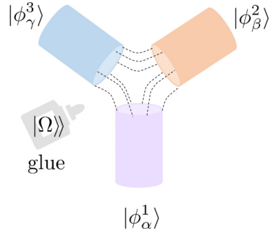
FIG. 11. Wave-function overlap of three cylinders with the same circumference. The maximally-entangled state |\Omega\rangle acts as a “glue” to form the path integral on the Riemann surface.
