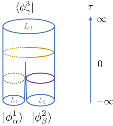
FIG. 1. The path integral for the wave-function overlap A_{\alpha\beta\gamma} = \langle \phi_\gamma^3 | \phi_\alpha^1 \phi_\beta^2 \rangle . The geometry is a three-sided cylinder \Sigma with circumference L_1 + L_2 = L_3 .
