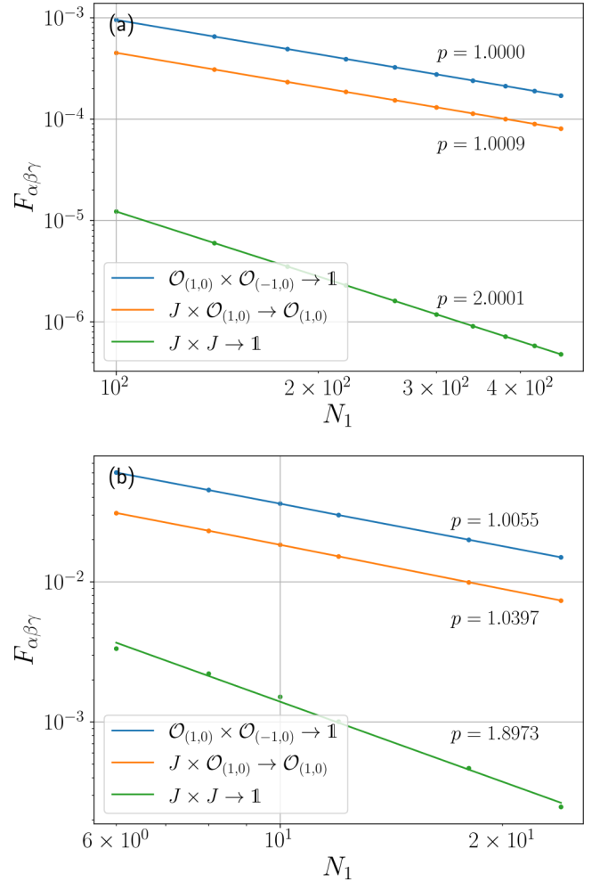
FIG. 5. Finite-size correction of wave-function overlap of the XXZ model at (a) \Delta = 0 and (b) \Delta = 1/2 , for the three channels under discussion. At the free fermion point \Delta = 0 , the system size is chosen in the range N_1 \in [100, 500] . The discrepancy between the theory and numerical value is less than 0.1%. At \Delta = 1/2 , we resort to tensor network method and the system size is chosen in the range N_1 \in [6, 24] . Due to the relatively small system size, the largest discrepancy is 5.1%.
