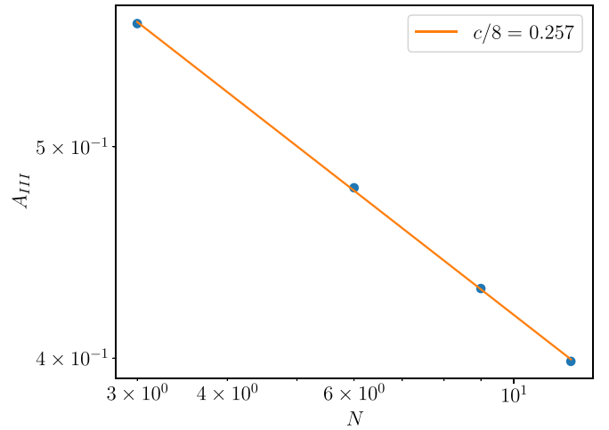
FIG. 7. Ground-state overlap A_{111} for the Haagerup model with N , N and 2N spins, where N = 3, 6, 9, 12 . The first two points are obtained by exact diagonalization, and the last two points are obtained by puMPS with maximal bond dimension D = 66 .
