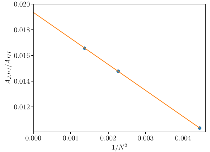
FIG. 9. A_{JJ^*\mathbb{1}}/A_{111} for the Haagerup model. In A_{JJ^*\mathbb{1}} the three states are taken from the Haagerup model with sizes 3n + 1 , 3n + 2 and N = 6n + 3 . In A_{111} , the three states are taken from the Haagerup model with sizes 3n , 3n + 3 and N = 6n + 3 . The three points in the plot correspond to n = 2, 3, 4 .
