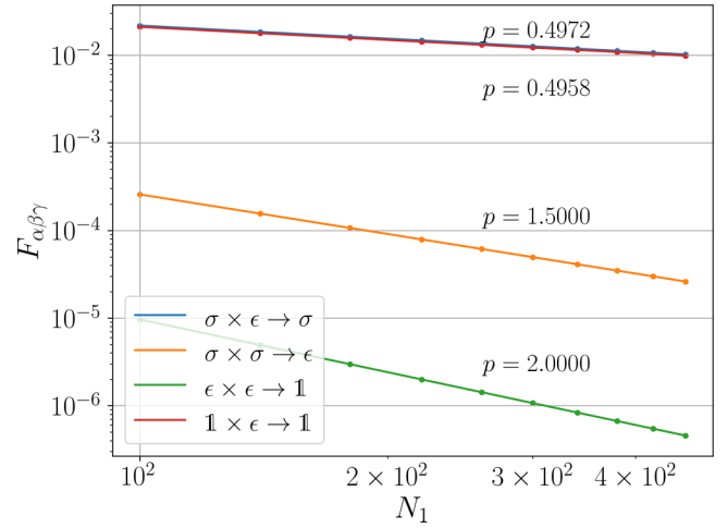
FIG. 4. Finite-size corrections of wave-function overlap in the critical Ising model, for the four channels: \sigma \times \epsilon \rightarrow \sigma , \sigma \times \sigma \rightarrow \epsilon , \epsilon \times \epsilon \rightarrow \mathbb{1} , \mathbb{1} \times \epsilon \rightarrow \mathbb{1} under discussion. The powers of leading finite-size corrections are p = \frac{1}{2}, \frac{3}{2}, 2, \frac{1}{2} , respectively, from the orbifold CFT. In the numerical computation we choose the system size N_1 \in [100, 500) , and we see the discrepancy between the theory and numerical value is less than 1%.
