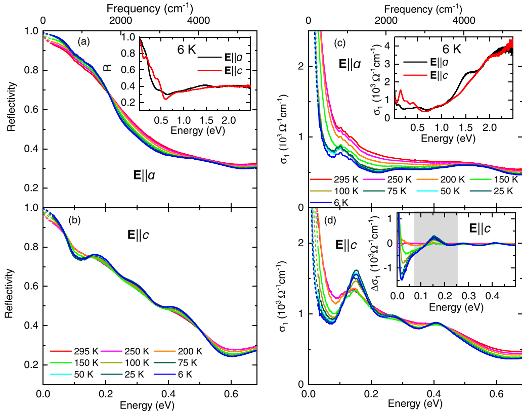
FIG. 2. Temperature-dependent reflectivity spectra of \text{Nb}_3\text{SiTe}_6 for the polarization directions (a) \mathbf{E}||a and (b) \mathbf{E}||c . Inset of (a): comparison between the reflectivity spectra at 6 K for the two polarization directions over a broad frequency range. (c), (d) Temperature-dependent optical conductivity \sigma_1 spectra of \text{Nb}_3\text{SiTe}_6 for \mathbf{E}||a and \mathbf{E}||c , respectively. Inset of (c): comparison between the \sigma_1 spectra at 6 K for the two polarization directions in the entire measured range. Inset of (d): difference spectra \Delta\sigma_1 calculated according to \Delta\sigma_1(\omega, T) = \sigma_1(\omega, T) - \sigma_1(\omega, 295 \text{ K}) . The gray area marks the full-width at half-maximum of the L1 peak at 295 K.
