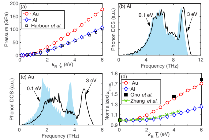
FIG. 4. (a) Comparison of electron temperature dependence of pressure in Au and Al. The hollow black squares denote variation of internal pressure with increase in electron temperature as reported by Harbour et al. [60]. Variations in the phonon density of states in (b) Al and (c) Au at electron temperatures of 0.1 (shaded region) and 3 eV (solid lines). (d) Variations in the maximum phonon frequency with electron temperature for Au and Al. We plot the normalized maximum frequency with respect to the maximum frequency at k_B T_e = 0 eV for Au and Al. The increase in pressure in Au is higher than that in Al with increasing electron temperatures, which translates to a greater phonon hardening effect in Au. We compare the normalized maximum frequencies for the metals with prior finite-temperature DFT calculations from Ono et al. [49] for Au and Zhang et al. [55] for Al.
