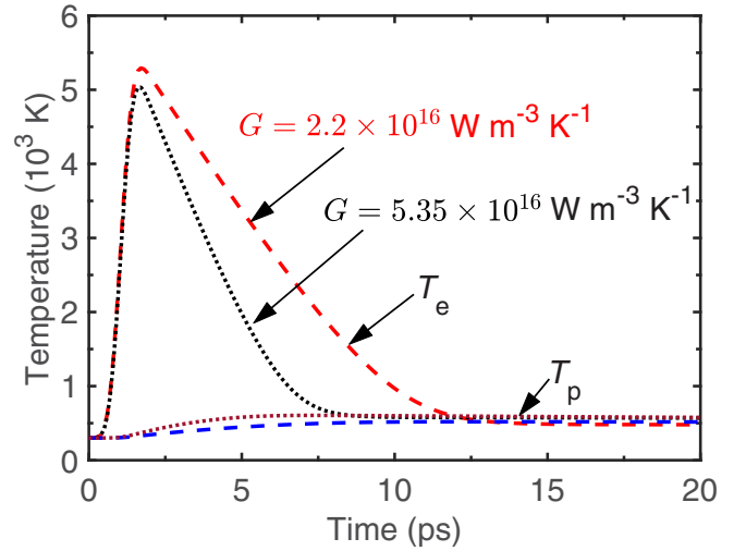
FIG. 11. Comparison of temperature profiles obtained by solving the modified TTM. The red dashed line indicates the temperature profile obtained using the room temperature e-p coupling factor of G = 2.2 \times 10^{16} \text{ W m}^{-3} \text{ K}^{-1} and the black dotted line indicates the temperature profile obtained using the calculated e-p coupling factor of G = 5.35 \times 10^{16} \text{ W m}^{-3} \text{ K}^{-1} at electron temperature of 0.5 eV.
