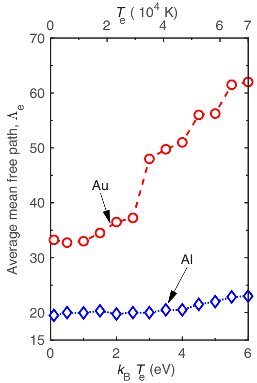
FIG. 7. Average mean-free paths, \Lambda_e , at the Fermi energy for Al and Au as a function of electron temperature. For Au, \Lambda_e increases with increase in electron temperature. However, for Al, the increase in \Lambda_e with electron temperature is much less pronounced, which is a direct consequence of the relatively different responses of the electron-phonon mass enhancement parameter of the two metals as shown in Fig. 5.
