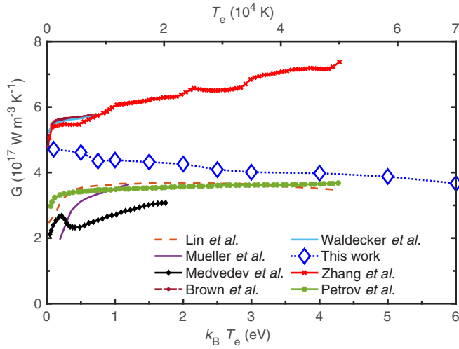
FIG. 10. Comparison of G(T_e) obtained from our calculation for Al with various theoretically reported values. Theoretically reported values include those of Zhang et al. [55], Brown et al. [15], Mueller et al. [76], Lin et al. [38], Medvedev et al. [75], Waldecker et al. [77], and Petrov et al. [73].
