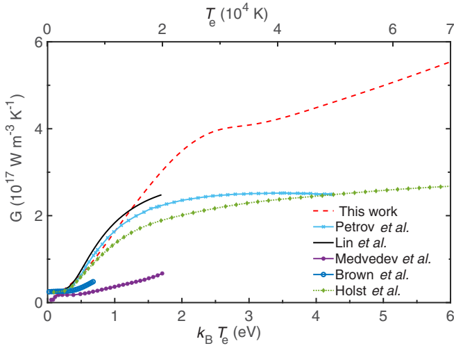
FIG. 9. Comparison of G(T_e) obtained from our calculation for Au with various theoretically reported values. Theoretically reported values include those of Petrov et al. [73], Lin et al. [38], Holst et al. [74], Medvedev et al. [75], and Brown et al. [15].
