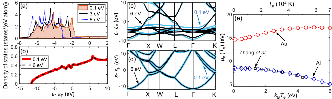
FIG. 1. Electronic density of states for (a) Au and (b) Al at varying electron temperatures as obtained from parameter-free density functional theory calculations. Electronic band structures for (c) Au and (d) Al at electron temperatures of 0.1 eV and 6 eV. (e) Variation in the chemical potential for Au and Al with increasing electron temperatures. The hollow black squares denote the finite-temperature DFT calculations of the chemical potential for Al as reported by Zhang et al. [55]. The agreement between our results and that of Zhang et al. [55] provides confidence in our results of the electronic structure calculations.
