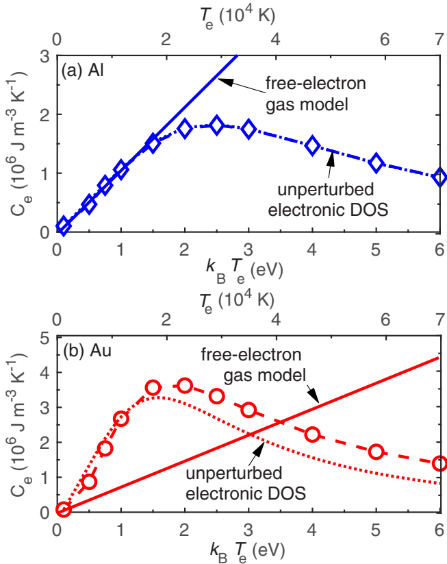
FIG. 3. Temperature-dependent heat capacities C_e(T_e) , calculated as a function of electron temperature, for (a) Al and (b) Au. For comparison, we also plot the predictions from the simplified free-electron model along with predictions of Eq. (9) that utilizes the unperturbed electronic density of states (calculated at T_e = 0 K). For Al, the free-electron gas model agrees well with our parameter-free calculations at lower temperatures, whereas it significantly underpredicts our DFT-based calculations at higher electron temperatures. For Au, the free-electron gas model can not predict the temperature dependence of the heat capacity for the entire temperature range. Furthermore, for the case of Au, the use of the unperturbed electronic density of states also leads to erroneous calculations of heat capacity, especially at higher electron temperatures.
