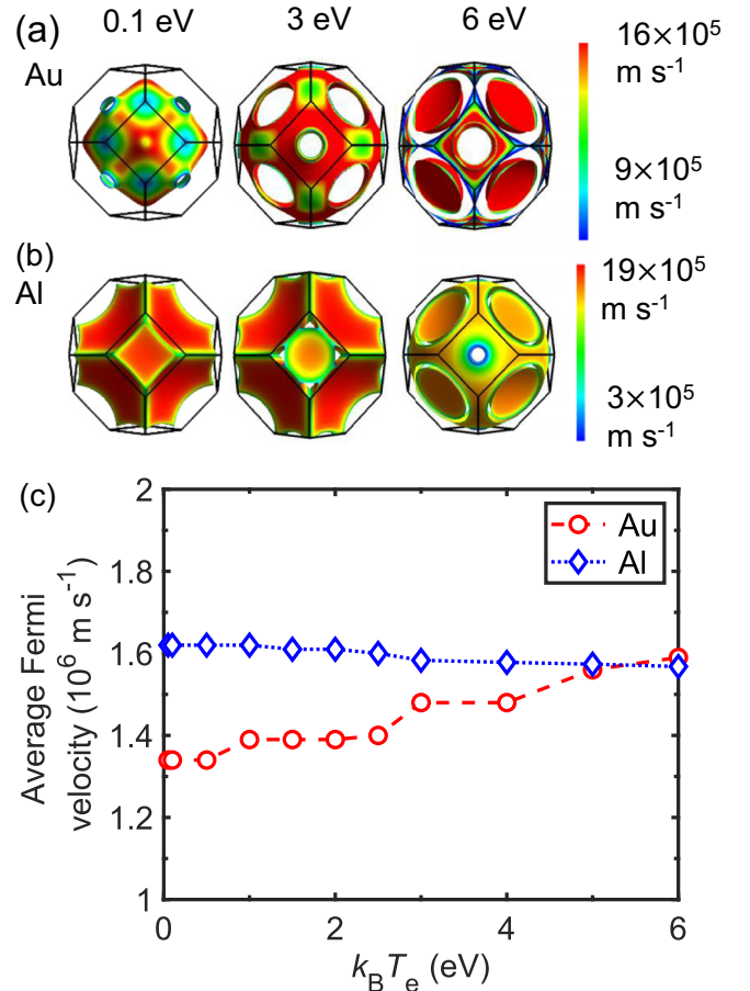
FIG. 2. Evolution of Fermi surfaces for (a) Au and (b) Al at three different electron temperatures. Color represents the variation in Fermi velocities at the Fermi surface. (c) Average Fermi velocity plotted as a function electron temperature. The Fermi velocity increases for Au while for Al, it has a slight decrease over the entire temperature range.
