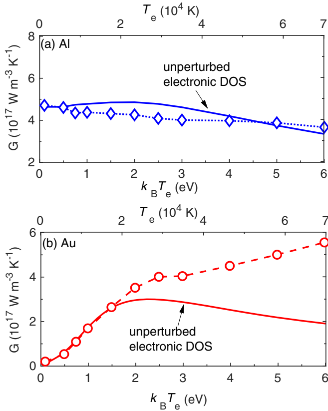
FIG. 6. Comparison of calculated volumetric electron-phonon coupling factor, G(T_e) , for (a) Al and (b) Au. The solid lines represent calculations of G(T_e) obtained from Eq. (9) by utilizing the electronic DOS and the second moment of phonon spectrum, \langle \omega^2 \rangle , obtained from the calculations of the unperturbed ( T_e = 0 K) case.
