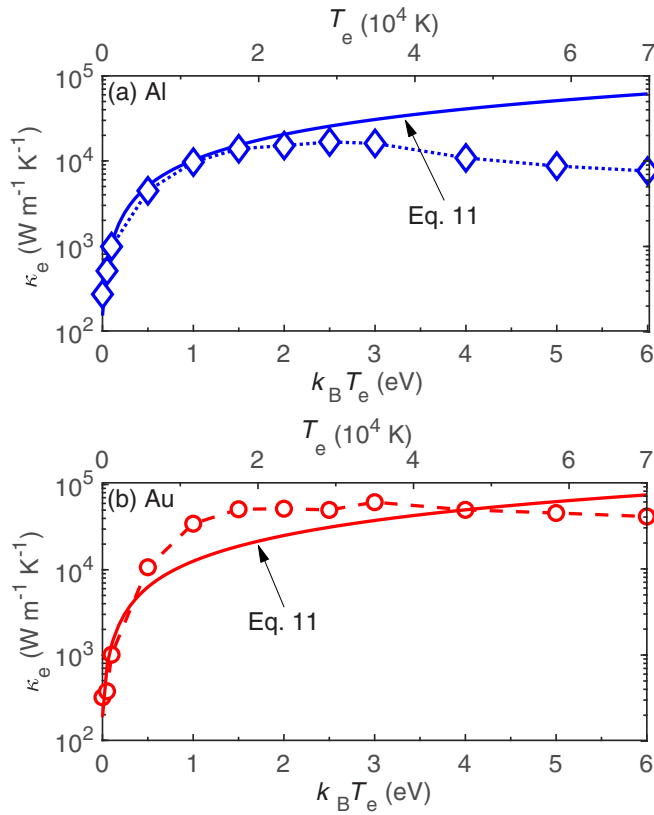
FIG. 8. (a) Electron temperature-dependent thermal conductivities, \kappa_e(T_e) , for (a) Al and (b) Au. The solid lines represent calculations from a simplified semiempirical model as given by Eq. (11).
