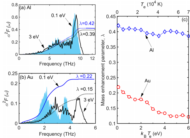
FIG. 5. (a) Eliashberg spectral functions, \alpha^2 F(\omega) , for (a) Al and (b) Au at electron perturbations of 0.1 and 3 eV. The solid and dotted lines represent the calculations of mass enhancement parameters ( \lambda ) at 0.1 and 3 eV, respectively. (c) Mass enhancement parameter as a function of electron temperature for the two metals.
