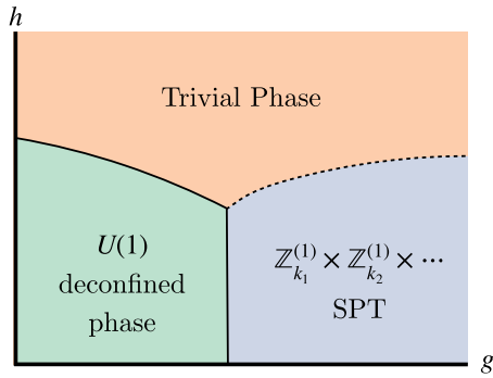
FIG. 2. The schematic phase diagram of the model described by Eq. (34) with the additional term contributing to the action amplitude e^{h \sum_{ij} a_{i,j}^{\mathbb{R}/\mathbb{Z}}} . When h = 0 , there are no fluctuations of U(1) gauge charge, and the model has an exact \mathbb{Z}_{k_1}^{(1)} \times \mathbb{Z}_{k_2}^{(1)} \times \dots 1-symmetry. For h \neq 0 , this becomes an exact emergent \mathbb{Z}_{k_1}^{(1)} \times \mathbb{Z}_{k_2}^{(1)} \times \dots 1-symmetry existing below the energy gaps of U(1) gauge charges, which exists in the green and purple shaded regions. Due to the 2\pi -quantized topological term, in the confined phase (shown in purple) there is an SPT order protected by the exact emergent \mathbb{Z}_{k_1}^{(1)} \times \mathbb{Z}_{k_2}^{(1)} \times \dots 1-symmetry whose SPT invariant is given by Eq. (70).
