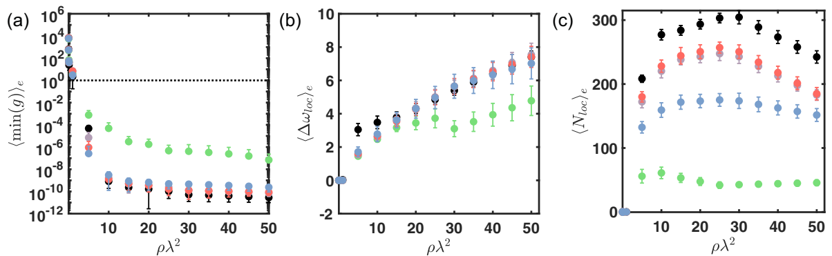
FIG. 8. (a) Trend of the minimum of the Thouless number as a function of \rho\lambda^2 . (b) Width of the frequency range \Delta\omega_{loc} for different optical densities where all the scattering resonances have a Thouless number lower than 1. (c) Number of localized scattering resonances as a function of \rho\lambda^2 . All these parameters are averaged with respect to 25 different realizations and the error bars are the statistical errors associated with this average ensemble operation. The pastel green, violet, red, and blue markers refer to point patterns generated with a probability p equal to [1,1,1,0], [1,1,0.75,0.5], [1,0.75,0.75,0.5], and [1,0.75,0.5,0.25], respectively. The black markers denote the UR structure.
