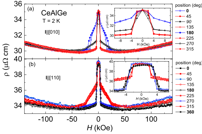
FIG. 7. Field-dependent resistivity of CeAlGe single crystals measured in the four-probe wire configuration at constant angles at 2 K (a) \mathbf{I}||[010] and (b) \mathbf{I}||[110] . Insets show zoom in of low-field data.
