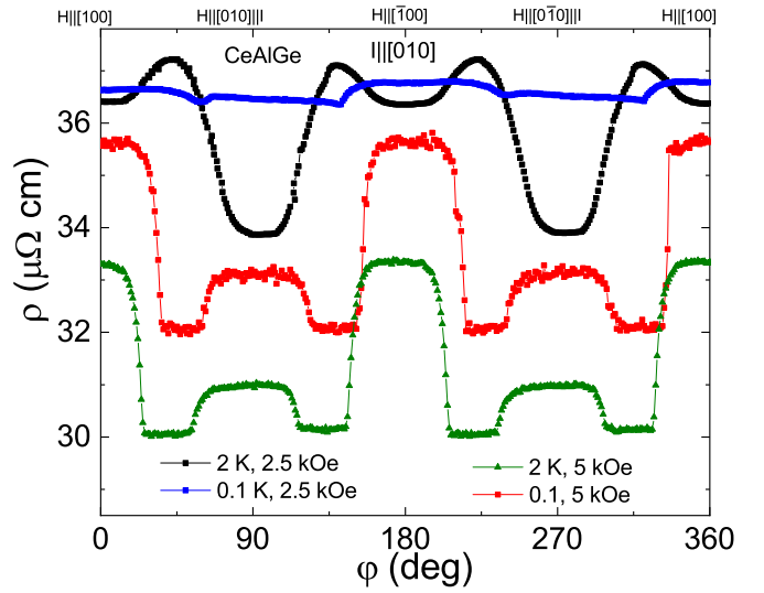
FIG. 5. Angle-dependent resistivity of CeAlGe single crystal measured in the four-probe wire configuration \mathbf{I}||[010] at T \leq 2 K for H = 2.5 and 5 kOe.
