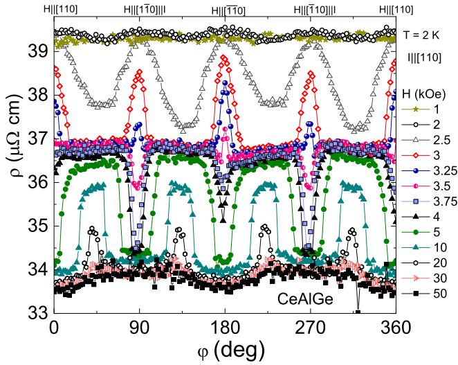
FIG. 3. AMR of CeAlGe single crystal measured in the four-probe wire configuration at 2 K, \mathbf{I}||[110] . The AMR data are clearly split into two regimes at H = 3.5 kOe, a value of the phase transition between the two different magnetic states. Field-dependent resistivity of CeAlGe measured in the four-probe wire configuration at constant angles at 2 K.
