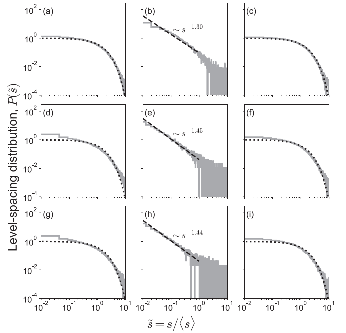
FIG. 8. Distribution of level spacing for the (a)–(c) Möbius, (d)–(f) Liouville, and (g)–(i) Legendre sequence structures. (a), (d), (g) Show the results obtained when considering all modes. (b), (e), (h) Show the results when analyzing single-peak modes only, whereas (c), (f), (i) when analyzing multi-peak modes only. The dotted lines correspond to the Poisson distribution P(\tilde{s}) = e^{-\tilde{s}} . The dashed lines are best fits with the indicated models. For this analysis we considered a large system with N = 10^5 sites.
