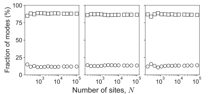
FIG. 6. Fraction of modes as a function of the number of sites N for the Möbius, Liouville, and Legendre sequence structures, respectively. Circles (squares) correspond to single-peak (multipeak) modes.
