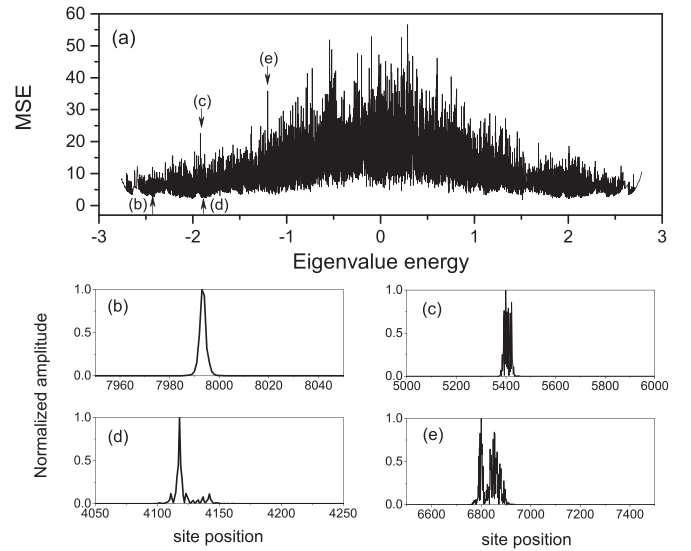
FIG. 5. (a) Mode spatial extent (MSE) of the Möbius structure. The arrows and corresponding letters label representative localized modes shown in (b)–(e) selected from the single-peak (b), (d) and multipeak (c), (e) populations.
