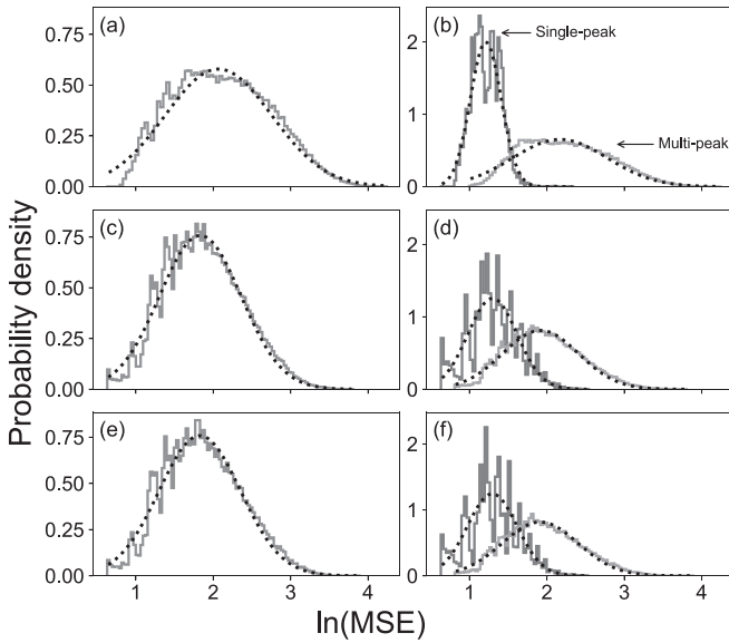
FIG. 7. Probability density of the logarithm of the MSE values of the eigenmodes for the (a), (b) Möbius, (c), (d) Liouville, and (e), (f) Legendre sequence structures. (a), (c), (e) Consider all the modes while (b), (d), (f) show the results for the two types of identified modes separately. The dotted lines are Gaussian fits. For this analysis we considered a large system with N = 10^5 sites.
