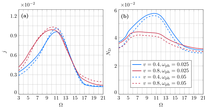
FIG. 7. (a) Time-averaged steady-state current j and (b) double occupancy N_D as a function of \Omega , for v = 0.4, 0.8 , at phonon cutoff frequencies \omega_{\text{ph}} = 0.025, 0.05 . Default parameters are specified at the beginning of Sec. IV.
