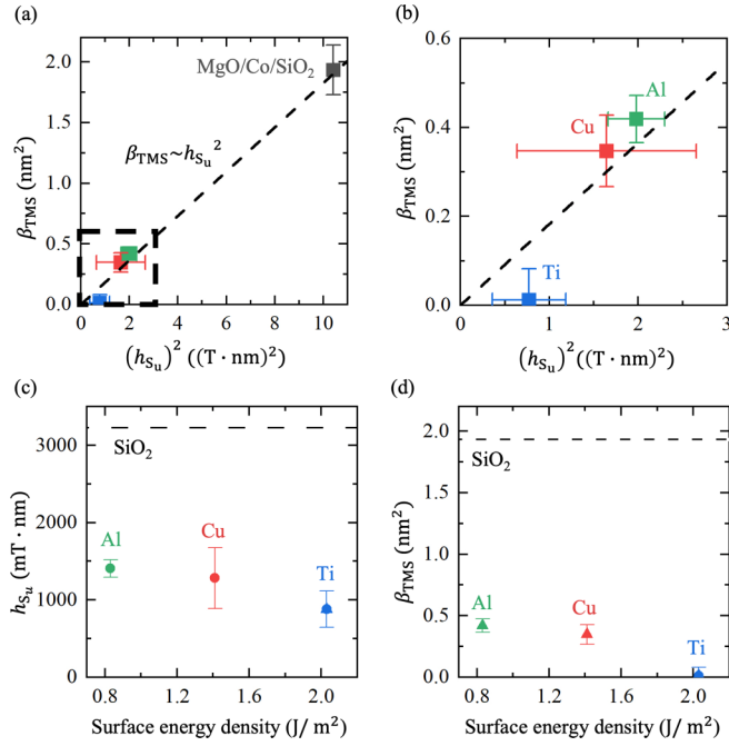
FIG. 4. (a) Correlation diagram between the TMS coefficient \beta_{\text{TMS}} and the square of the SMA field (h_{\text{su}})^2 . The broken line indicates the fitting result for the samples with the NM seeding layers. In the correlation between \beta_{\text{TMS}} and (h_{\text{su}})^2 , the blue, red, green, and black points represent the data points for Co/Ti, Co/Cu, Co/Al, and Co/SiO 2 , respectively. (b) The enlarged figure in the block broken square. Surface energy density dependence of the NM materials selected as the seeding layers on (c) \beta_{\text{TMS}} and (d) h_{\text{su}} , where the black broken lines in (c) and (d) show the values of the MgO/Co/SiO 2 .
