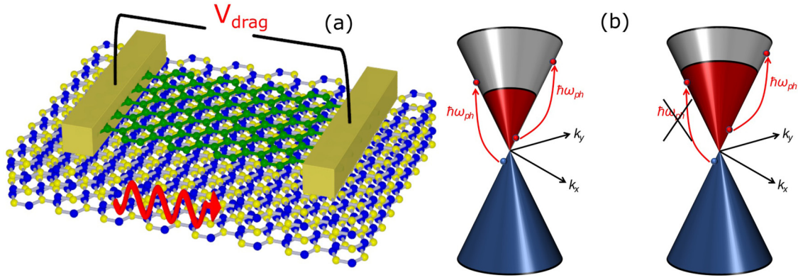
FIG. 1. (a) Schematic representation of a stacked heterostructure of graphene (green bonds) and hBN (gray bonds) that exploits the phonon-drag effect for phonon (red arrow) detection. (b) Phase space for electron excitation via e-SPP interaction in monolayer graphene. When E_F < \hbar\omega_{ph} , there are two possible kinds of excitation: Interband (valence to conduction band) and intraband (within the conduction band). When E_F > \hbar\omega_{ph} , the interband transition is no longer allowed.
