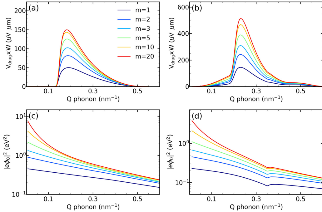
FIG. 3. Phonon drag voltage V_{\text{drag}} as a function of a hBN SPP wave vector in (a) monolayer and (b) bilayer graphene. Results are shown for different hBN layer number m , or thickness t_{\text{hBN}} = m \times 3.4 \text{ \AA} . Panels (c) and (d) depict the e-SPP scattering potential from Eq. (A10) for monolayer and bilayer graphene, respectively. The weak kink at Q = 0.34 \text{ nm}^{-1} in panel (d) is due to the polarization function anomaly at Q = 2k_F [45,46]. The calculations assume T = 50 \text{ K} and n = 10^{12} \text{ cm}^{-2} .
