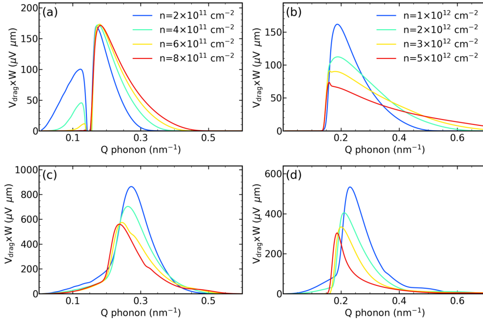
FIG. 2. Phonon drag voltage V_{\text{drag}} as a function of the hBN SPP wave vector, and for various carrier densities in the graphene layer. Panels (a) and (b) show results for monolayer graphene, while panels (c) and (d) are for bilayer graphene. The legend of panel (a) applies to panel (c) also, while that of panel (b) applies to panel (d). The calculations assume T = 50 K and t_{\text{hBN}} = \infty .
