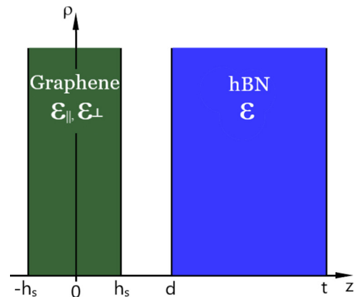
FIG. 6. Schematic illustration of the cross section of the graphene/hBN heterostructure. The monolayer or bilayer graphene is taken to be of thickness 2h_s , with an anisotropic dielectric function ( \varepsilon_{\perp}, \varepsilon_{\parallel}(q) ) and centered around z = 0 . The hBN of thickness t_{\text{hBN}} = t - d , and dielectric function \varepsilon(\omega) , supports the SPP.
