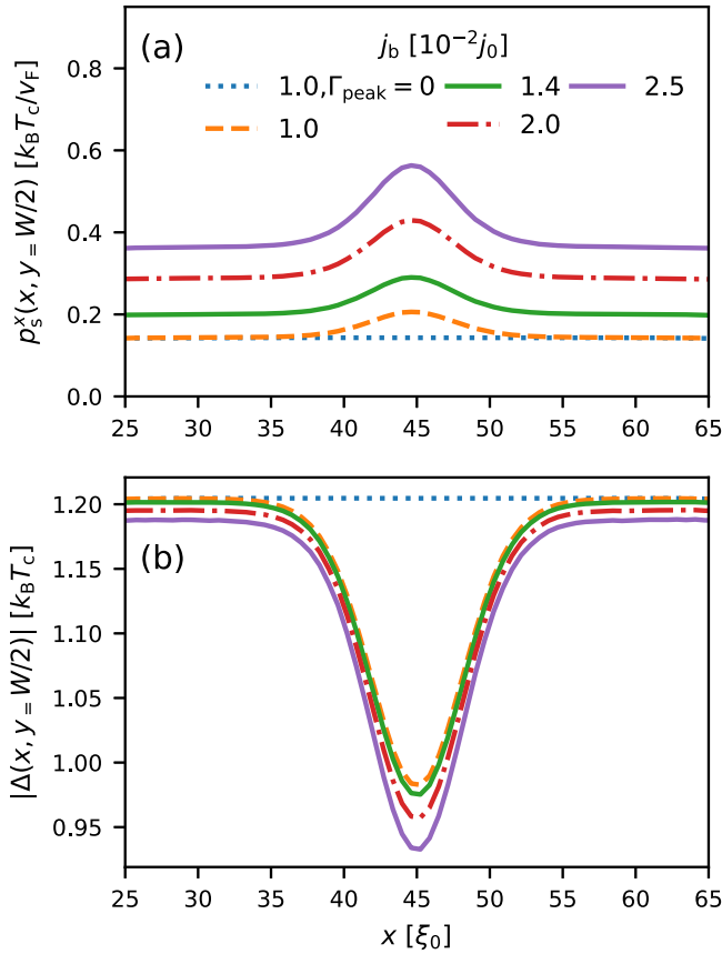
FIG. 12. Variation of the superconducting order parameter along a line cut in the center of the channel, y \approx W_l/2 (see Fig. 8), for \Gamma_{\text{peak}} = 0 (dotted blue) and \Gamma_{\text{peak}} = 5 \times 10^{-2} \pi k_B T_c (other lines) at different values of the boundary current j_b . (a) The x component of the superflow \mathbf{p}_s^x = (\hbar/2) \partial_x \chi(x, y) and (b) the suppression of the order parameter in the groove.
