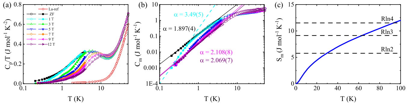
FIG. 4. (a) Specific heat of \text{PrZnAl}_{11}\text{O}_{19} measured at various magnetic fields. The open and closed symbols represent the data sets obtained in the He4 and dilution-refrigerator temperature regimes. The phonon contribution obtained from the renormalized \text{LaZnAl}_{11}\text{O}_{19} data is also shown. (b) Temperature dependence of the magnetic specific heat on a log-log scale. The lines are fits according to a power law, whose exponents are also shown. (c) The ZF magnetic entropy is obtained by integrating the magnetic specific-heat C_m/T .
