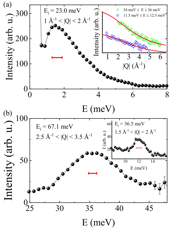
FIG. 3. Energy cuts at different |Q| positions. The red bars indicate the instrument energy resolution at the specific E position. The inset of (a) shows the |Q| dependence of the intensity for the 12- and 36-meV excitations, which follow the magnetic form factor of \text{Pr}^{3+} , |f(Q)|^2 , plus a small constant background.
