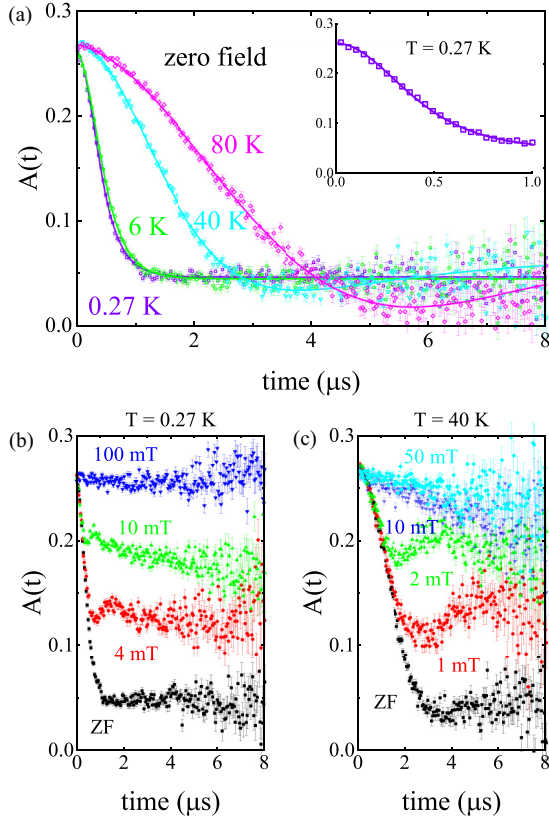
FIG. 5. (a) ZF- \mu SR spectra measured at various temperatures. The solid curves represent the fit as described in the text. (b) and (c) LF- \mu SR spectra measured at 0.27 and 40 K, respectively.
