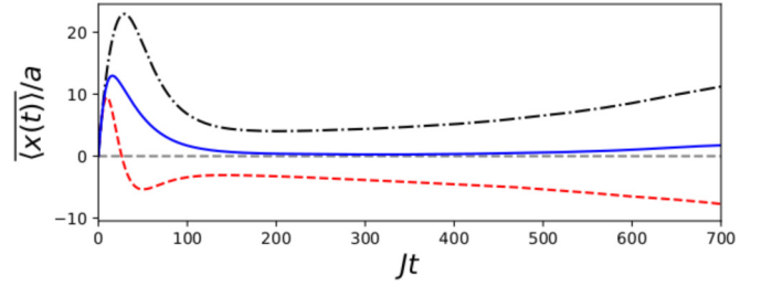
FIG. 7. Hatano-Nelson model with complex potential. We compute \overline{\langle x(t) \rangle}_> (black dot-dashed), \overline{\langle x(t) \rangle}_< (red dashed), and \overline{\langle x(t) \rangle} (blue solid line) using |J_a|/J = 0.01 , W/J = 0.5 , k_0 a = 1.4 , \sigma/a = 10 , N = 2 \times 10^3 , and n_d = 5 \times 10^5 . The model does not present the QBE.
