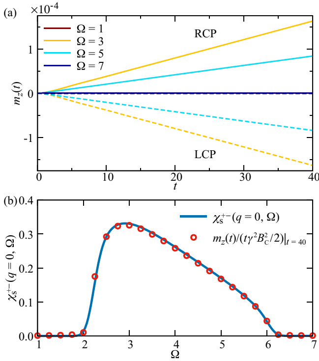
FIG. 2. (a) Time-dependent magnetization m_z(t) under the magnetic field \mathbf{B}(t) = B_C(\cos \Omega t, \pm \sin \Omega t) , where J = 1 , \Delta = 4 , and \hbar\gamma B_C = 0.005 ( \hbar/J is a unit of time). The solid and dotted lines indicate the magnetization under right-handed circularly polarized (RCP) and left-handed circularly polarized (LCP) fields, respectively. The data at \Omega = 1 and 7 are overlapped around m_z(t) \sim 0 . (b) Comparison between the dynamical spin structure factor \chi_s^{+-}(q=0, \Omega) (solid line) and the \Omega dependence of the magnetization normalized as m_z(t)/(t\gamma^2 B_C^2/2)|_{t=40} (circles).
