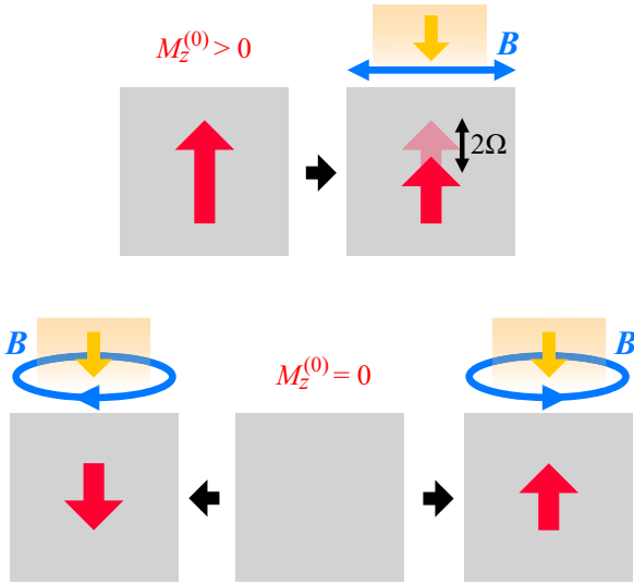
FIG. 1. Schematic pictures of the second-order magnetic effects. Top panel: Magnetization under the linearly polarized magnetic field when M_z^{(0)} > 0 in the ground state, where M_z^{(2)}(2\Omega) is activated. Bottom panel: Helicity-dependent magnetization under the circularly polarized magnetic fields when M_z^{(0)} = 0 .
