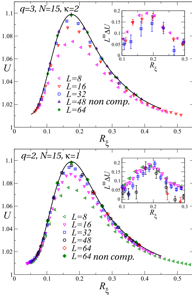
FIG. 5. Estimates of U versus R_\xi for the compact AH model with N = 15 and C^* boundary conditions. Top: Results for q = 3 and \kappa = 2 , bottom: results for q = 2 and \kappa = 1 ; The continuous line is an extrapolation of the data for the noncompact model [38]; noncompact-model data for L = 48 and L = 64 are also reported to provide an estimate of the accuracy of the extrapolation. The insets show the deviations from the extrapolated results: we report L^\omega \Delta U , where for each data point \Delta U = U - f_U(R_\xi) and f_U(R_\xi) is the extrapolation of the data for the noncompact model (continuous line in the main panels). We set \omega = 1 , but little changes if we decrease \omega as far as \omega \geq 0.6 .
